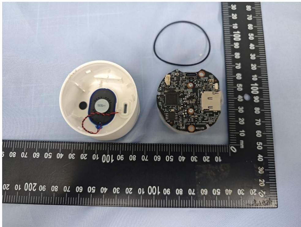
(6) EUT Photo (Tapo C120)
