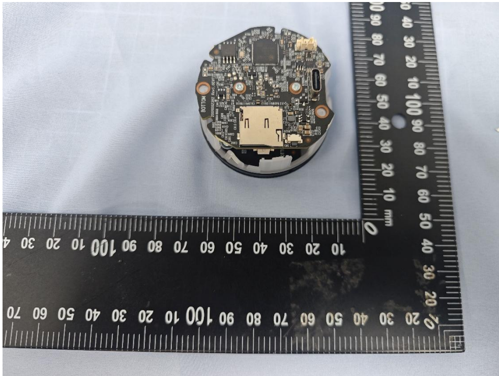
(24) EUT Photo (Tapo C121)
