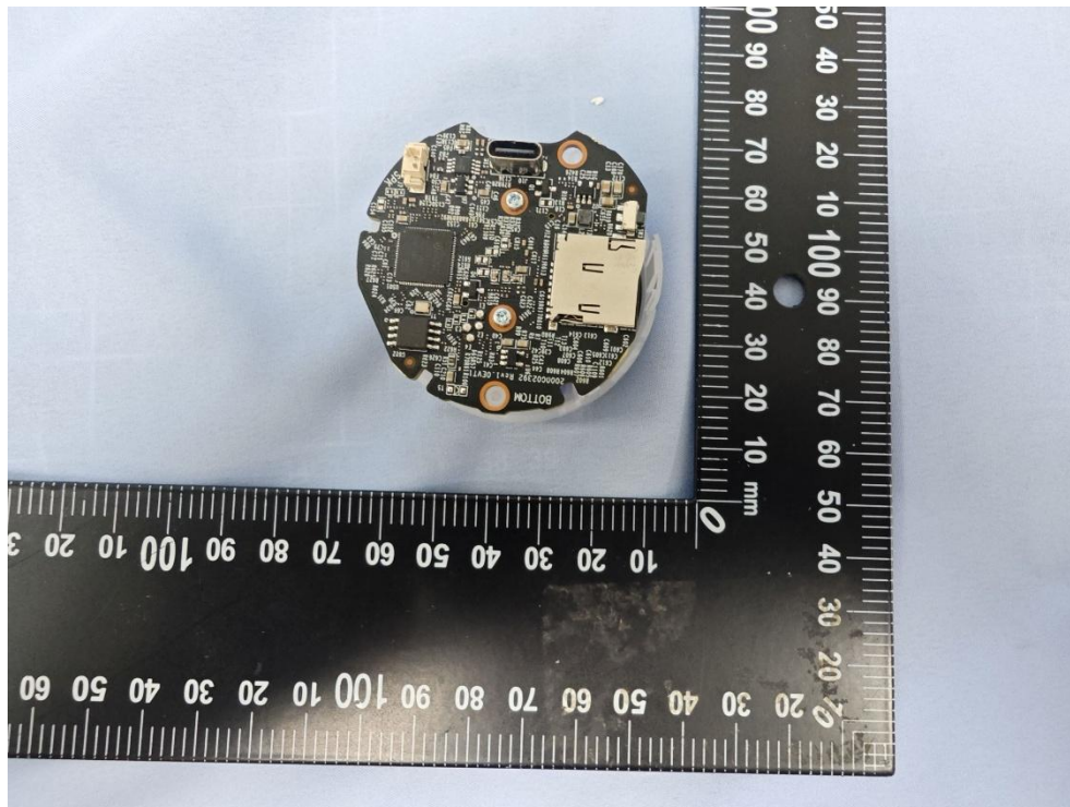
(8) EUT Photo (Tapo C120)
