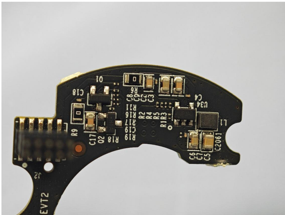
(36) EUT Photo (Tapo C121)
