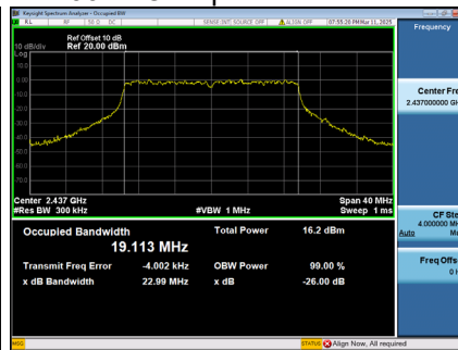
99 % Occupied Bandwidth
