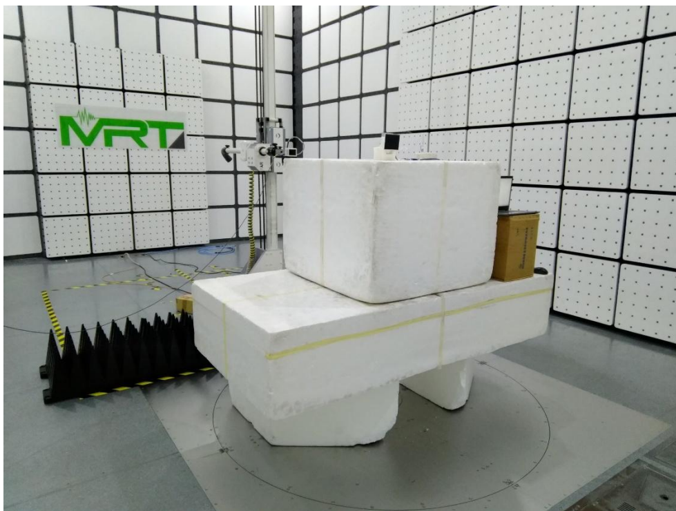
Description: Radiated Emission Test Setup for 9kHz~30MHz_BLE
