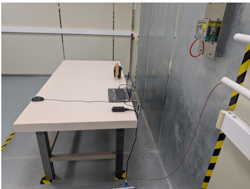
Description: Side View of Conducted Emission Test Setup (WiFi)
