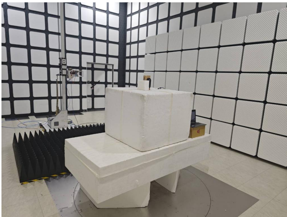
Description: Radiated Emission Test Setup for above 1GHz (BLE)
