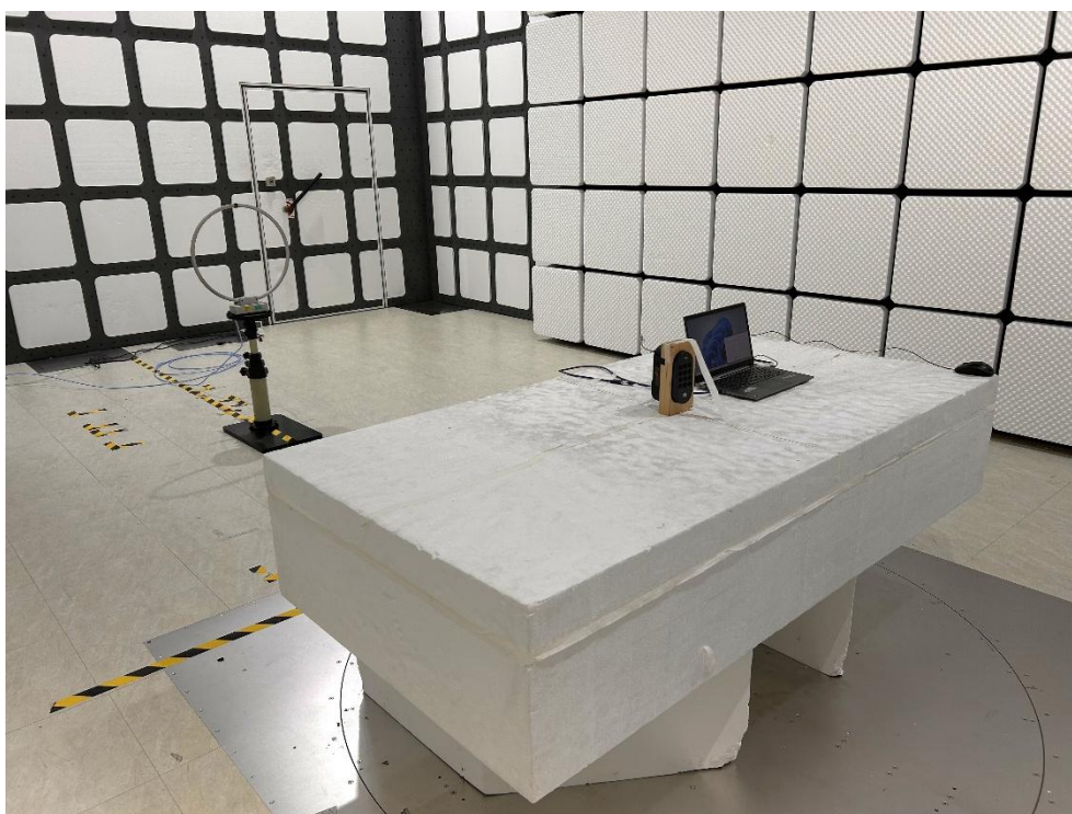
Description: Radiated Emission Test Setup for 9kHz~30MHz (WiFi)
