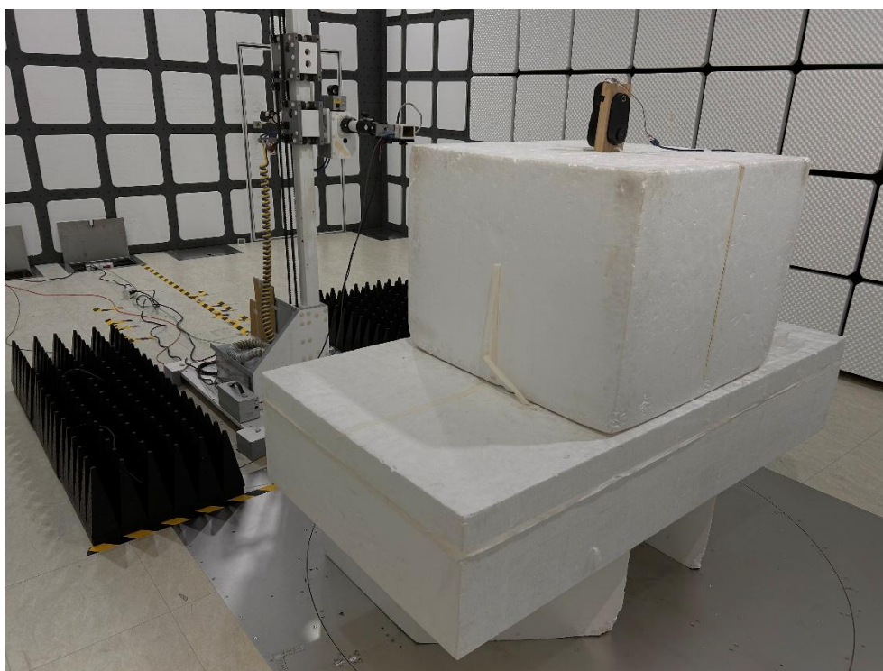
Description: Radiated Emission Test Setup for 9kHz~30MHz (WiFi)
