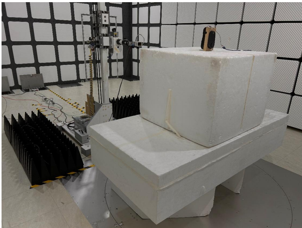
Description: Radiated Emission Test Setup for 9kHz~30MHz (BLE)
