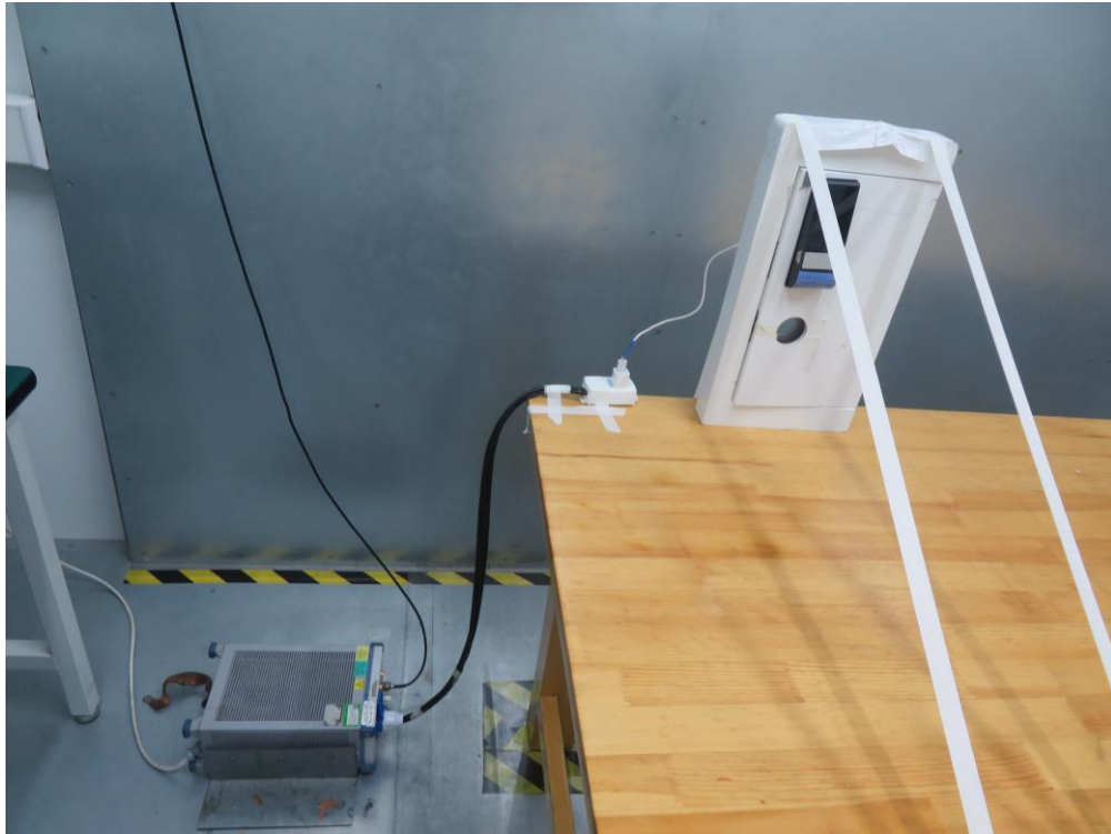
Description: Side View of AC Conducted Emissions Test Setup (SIP-SR2)
