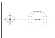
Measuring Template (For Door Lock)
