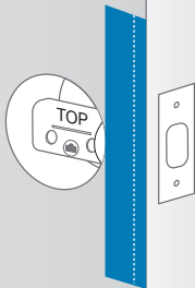
Backset 2-3/4" (70 mm)
