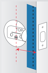
Backset 2-3/4" (70 mm)
