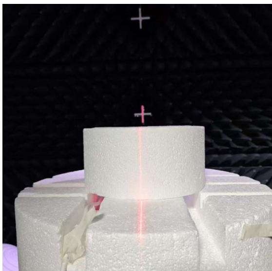
Figure 3-4 Antennas measurement diagram
