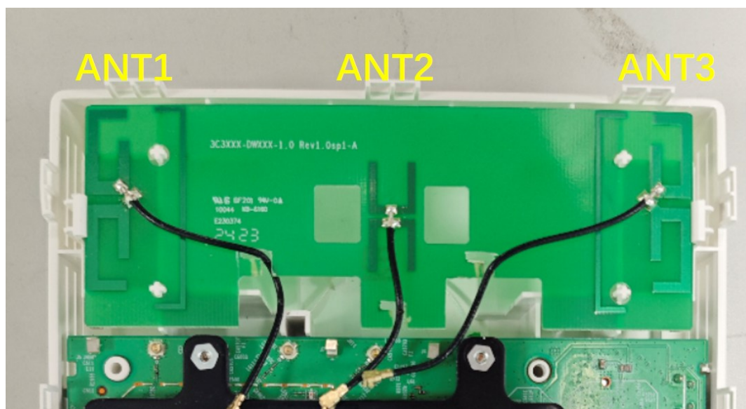
Figure 1-1 Locations of Antennas
