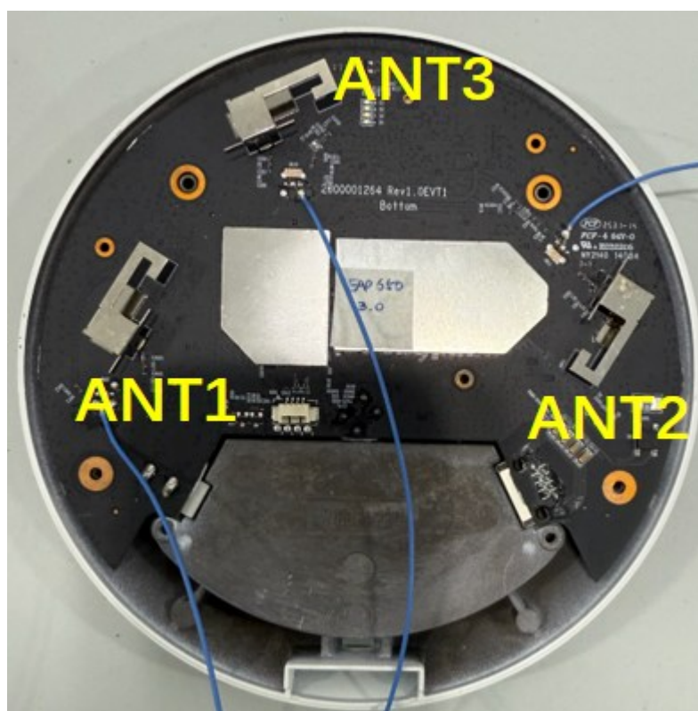
Figure 1-1 Locations of Antennas
