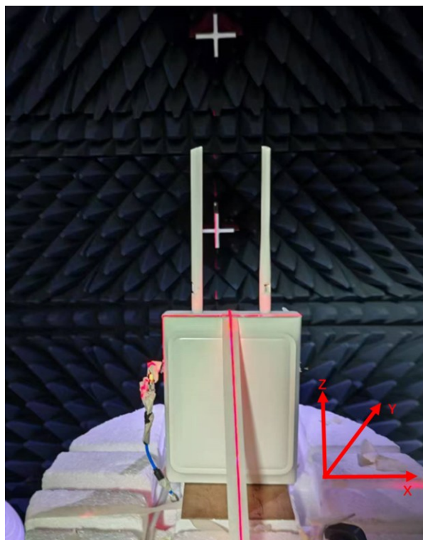
Figure 3-4 Antennas measurement diagram
