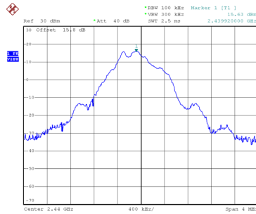
Reference Level-CH19
