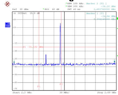
Bandedge-CH39
