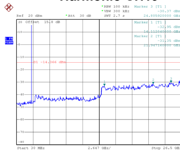
Harmonic-CH19
