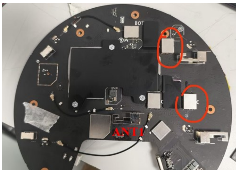
Figure 1-1 Locations of Antennas
