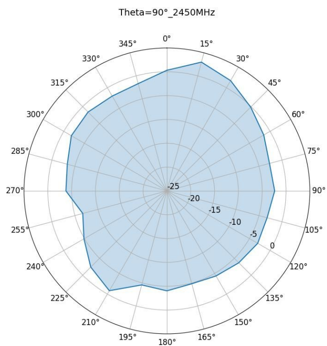
Ant3
