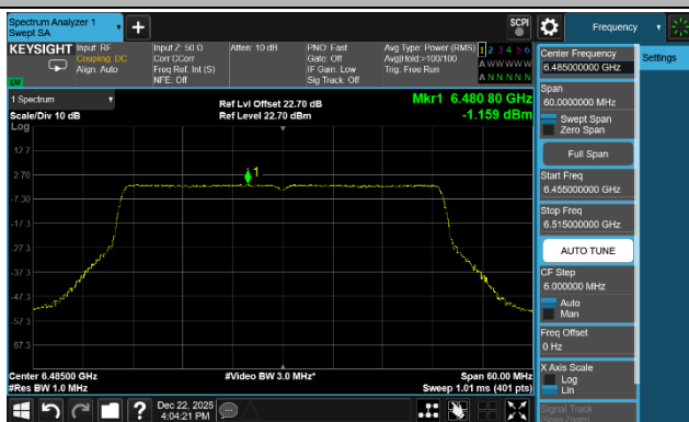
Channel 107 (6485 MHz)
