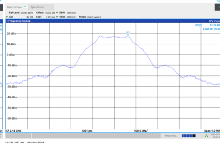
Bandedge-CH39
