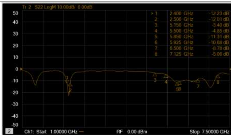
Ant3
