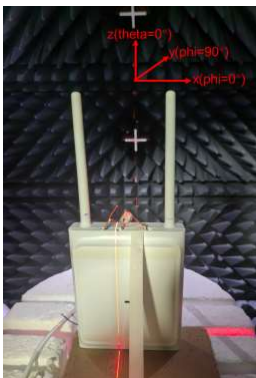
Figure 3-4 Antennas measurement diagram
