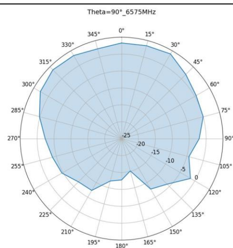
Ant5
