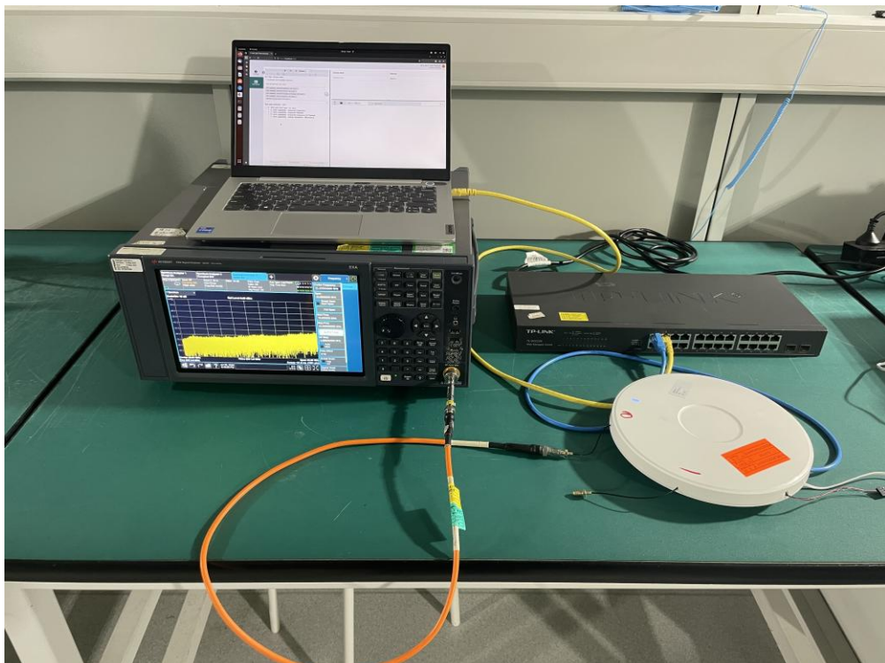
Description: AFC Test Setup
