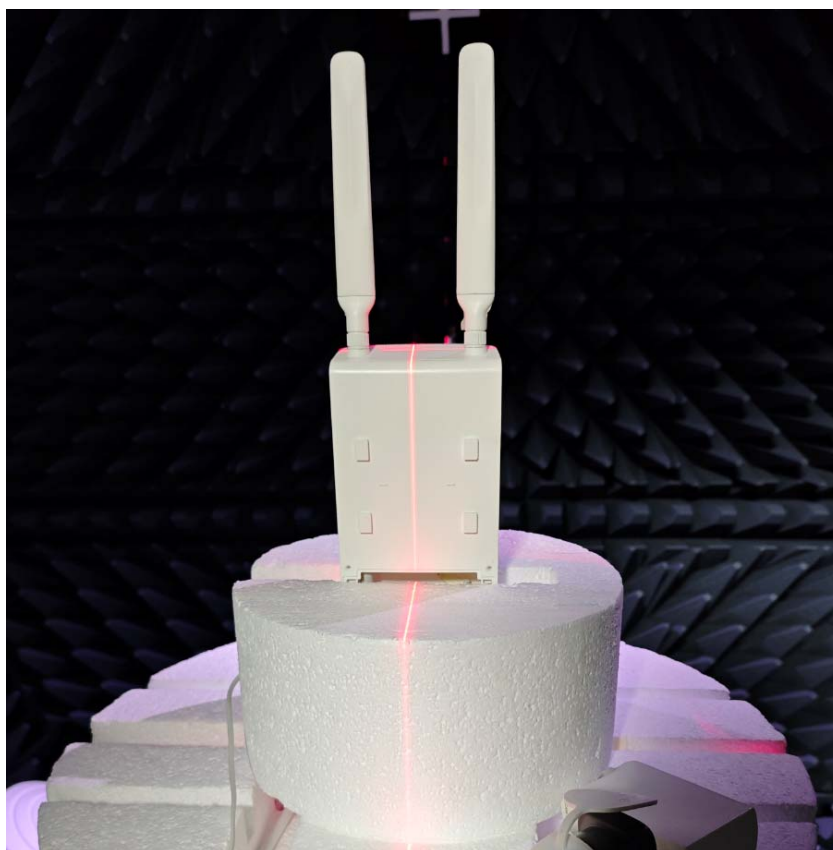
Figure 3-4 Antennas measurement diagram
