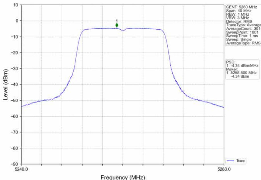
802.11a_LCH_5260MHz_Ant2_NTNV
