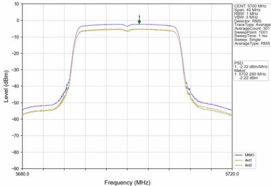
802.11ax(HE20)_HCH_5700MHz_RU242_Left_MIMO_NTNV
