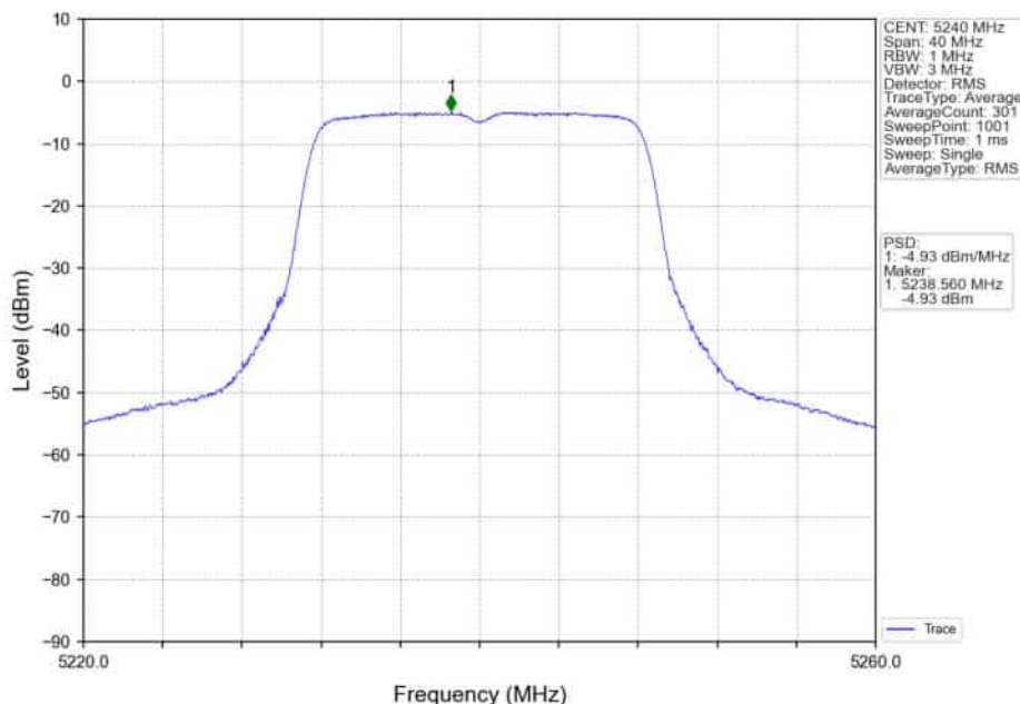
802.11a_HCH_5240MHz_Ant1_NTNV
