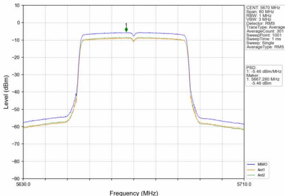
802.11ax(HE40)_HCH_5670MHz_RU484_Left_MIMO_NTNV
