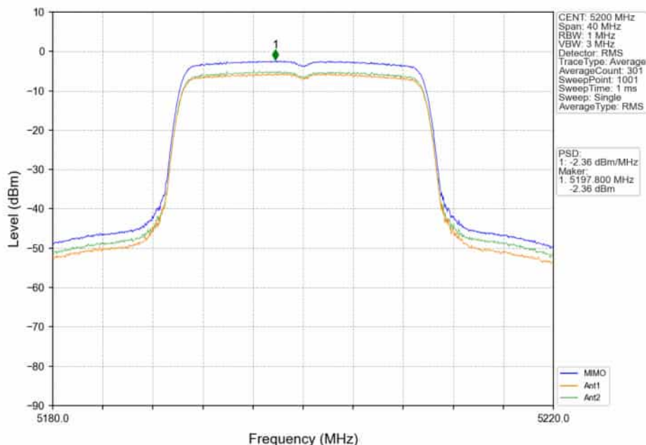
802.11ax(HE20)_MCH_5200MHz_RU242_Left_MIMO_NTNV
