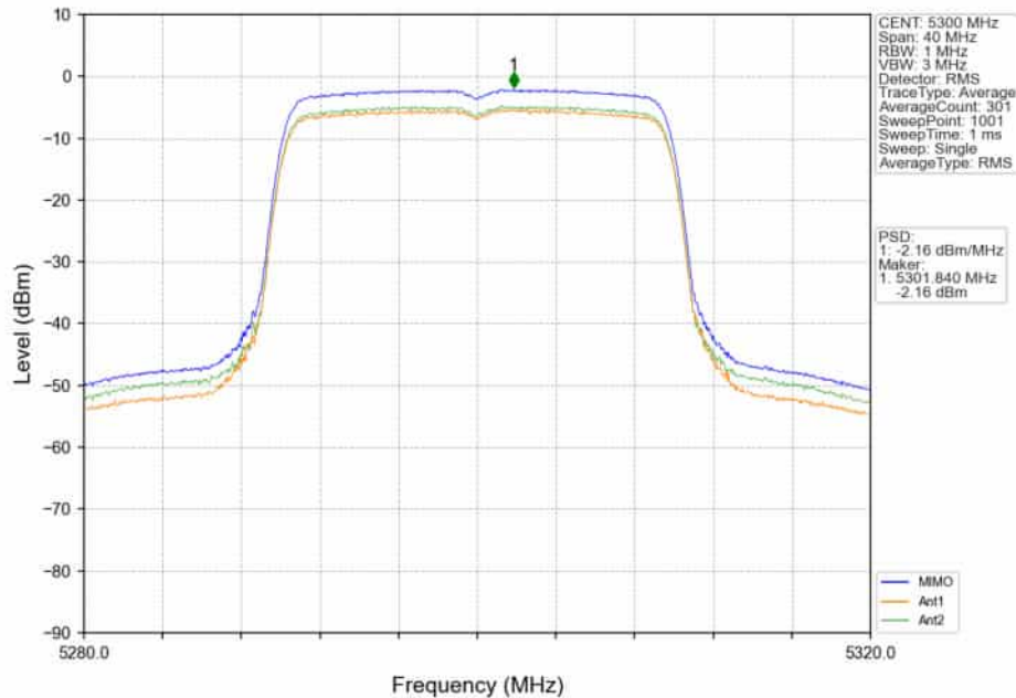
802.11ax(HE20)_MCH_5300MHz_RU242_Left_MIMO_NTNV
