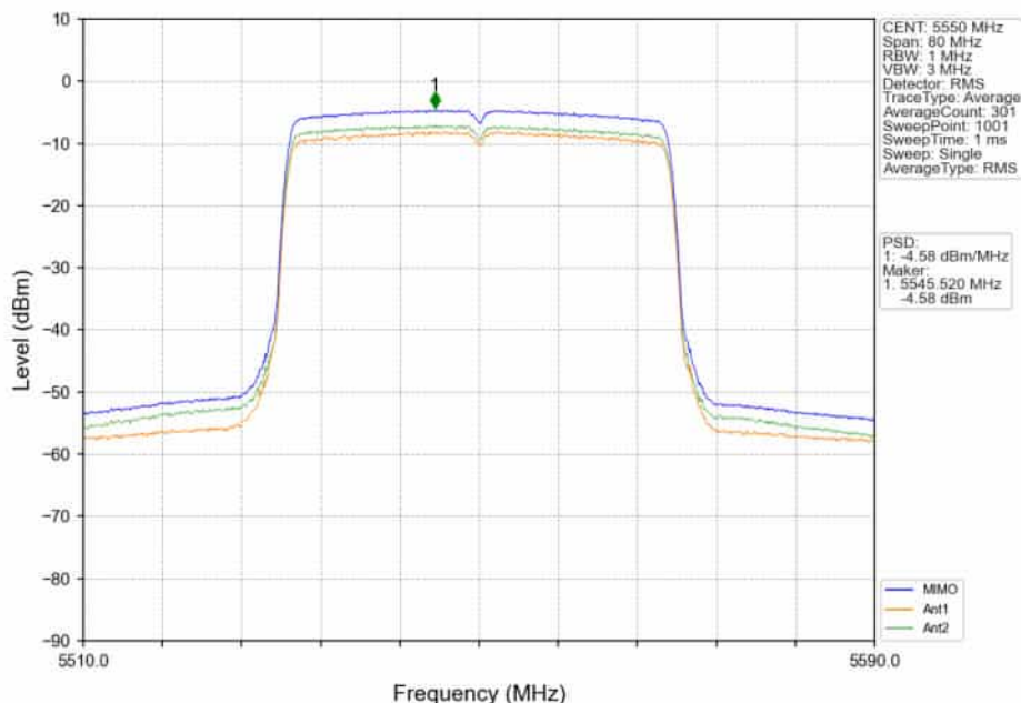
802.11ax(HE40)_MCH_5550MHz_RU484_Left_MIMO_NTNV
