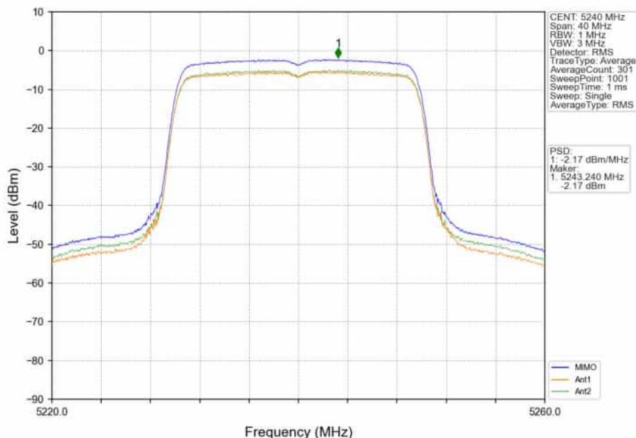
802.11ax(HE20)_HCH_5240MHz_RU242_Left_MIMO_NTNV
