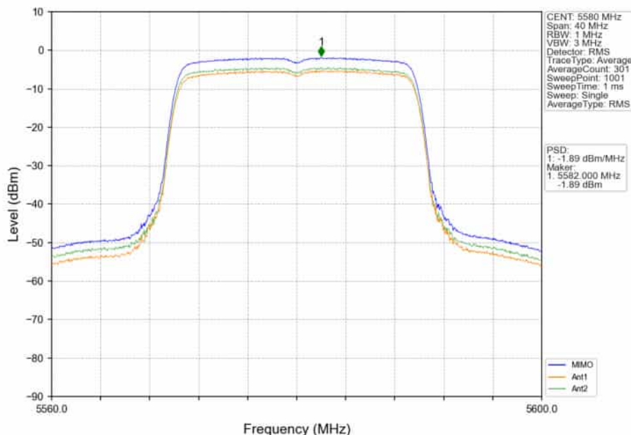
802.11ax(HE20)_MCH_5580MHz_RU242_Left_MIMO_NTNV
