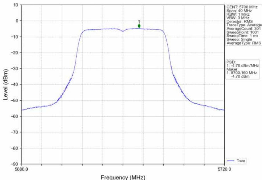
802.11a_HCH_5700MHz_Ant1_NTNV
