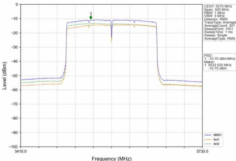
802.11ax(HE160)_MCH_5570MHz_2xRU996_Left_MIMO_NTNV
