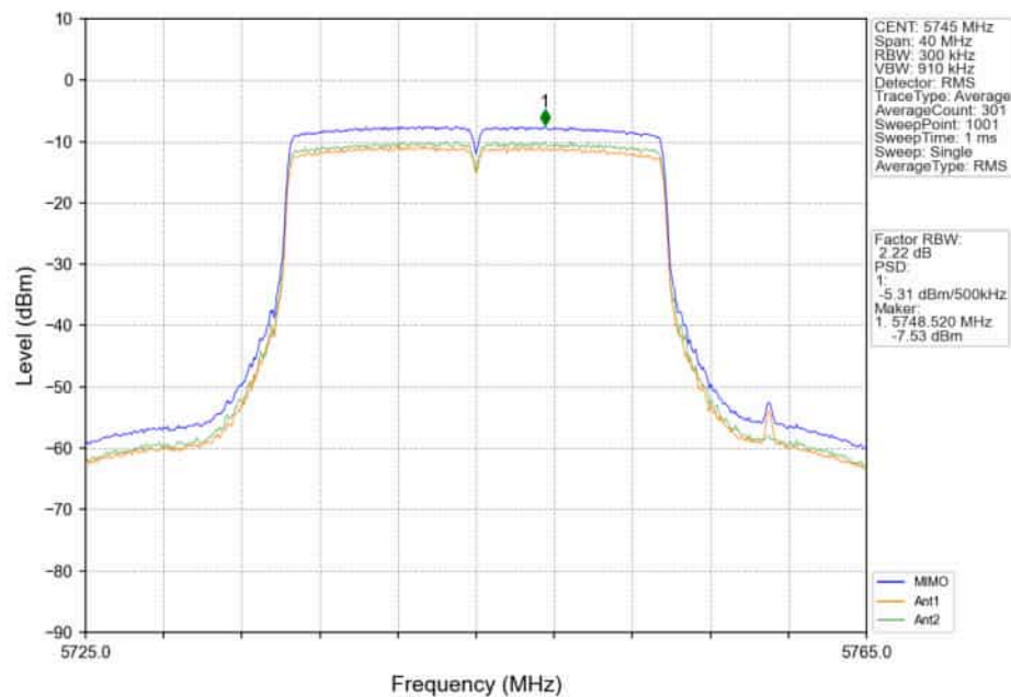
802.11ax(HE20)_LCH_5745MHz_RU242_Left_MIMO_NTNV
