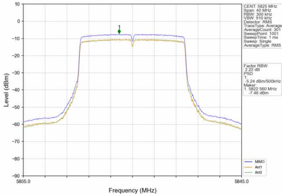
802.11ax(HE20)_HCH_5825MHz_RU242_Left_MIMO_NTNV
