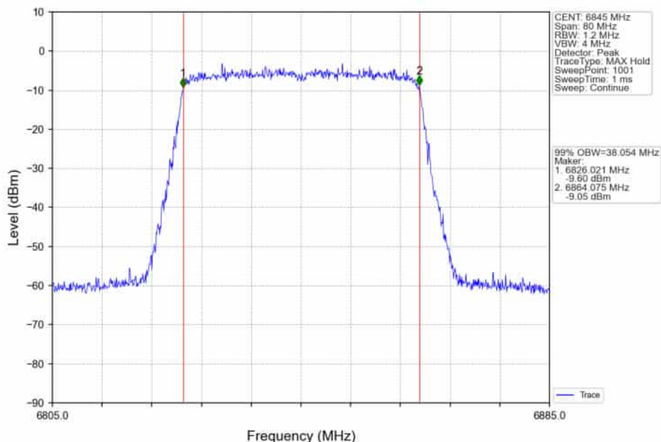
802.11ax(HEW40)_HCH_6845MHz_RU484_Left_Ant2_NTNV
