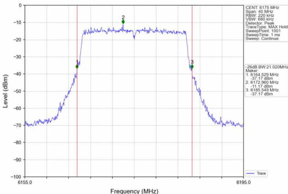
802.11ax(HEW20)_MCH_6175MHz_RU242_Left_Ant2_NTNV
