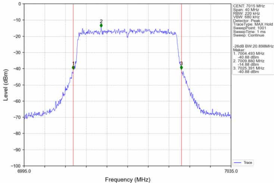
802.11ax(HEW20)_MCH_7015MHz_RU242_Left_Ant2_NTNV
