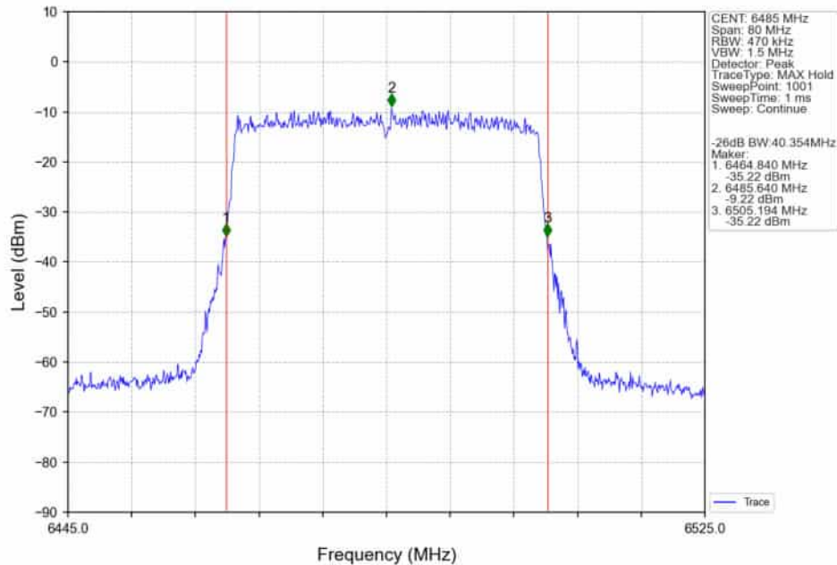
802.11ax(HEW40)_MCH_6485MHz_RU484_Left_Ant2_NTNV
