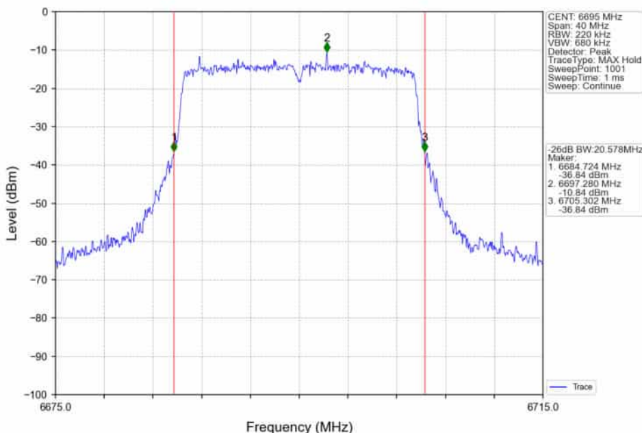
802.11ax(HEW20)_MCH_6695MHz_RU242_Left_Ant2_NTNV
