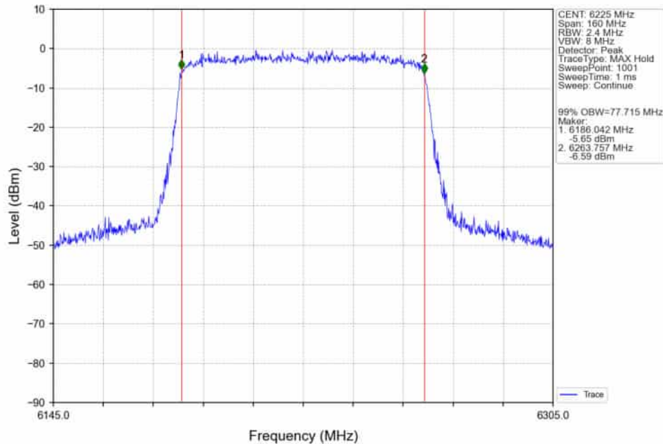
802.11ax(HEW80)_MCH_6225MHz_RU996_Left_Ant2_NTNV
