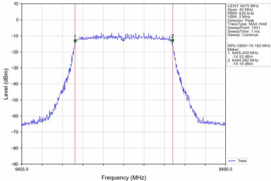
802.11ax(HEW20)_MCH_6475MHz_RU242_Left_Ant2_NTNV
