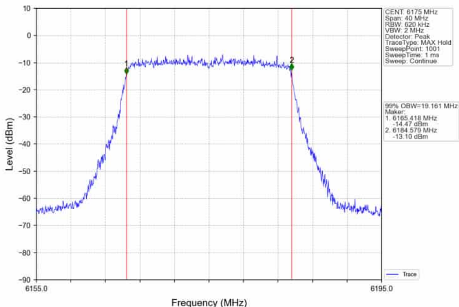
802.11ax(HEW20)_MCH_6175MHz_RU242_Left_Ant2_NTNV
