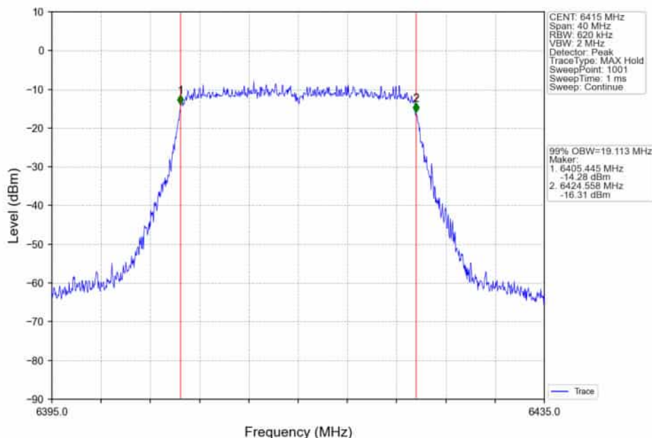
802.11ax(HEW20)_HCH_6415MHz_RU242_Left_Ant2_NTNV
