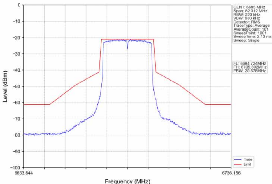
802.11ax(HEW20)_MCH_6695MHz_RU242_Left_Ant2_NTNV
