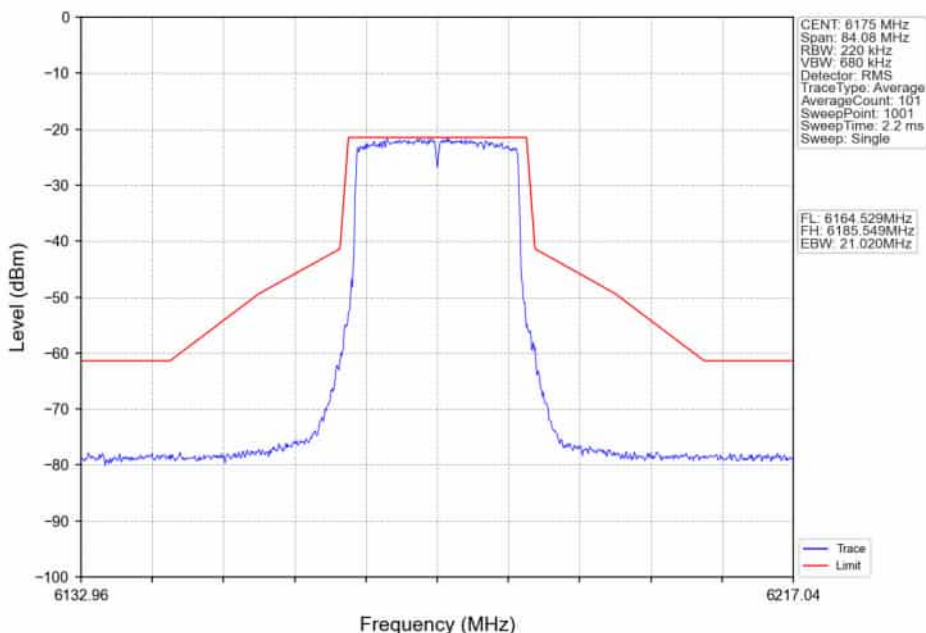
802.11ax(HEW20)_MCH_6175MHz_RU242_Left_Ant2_NTNV
