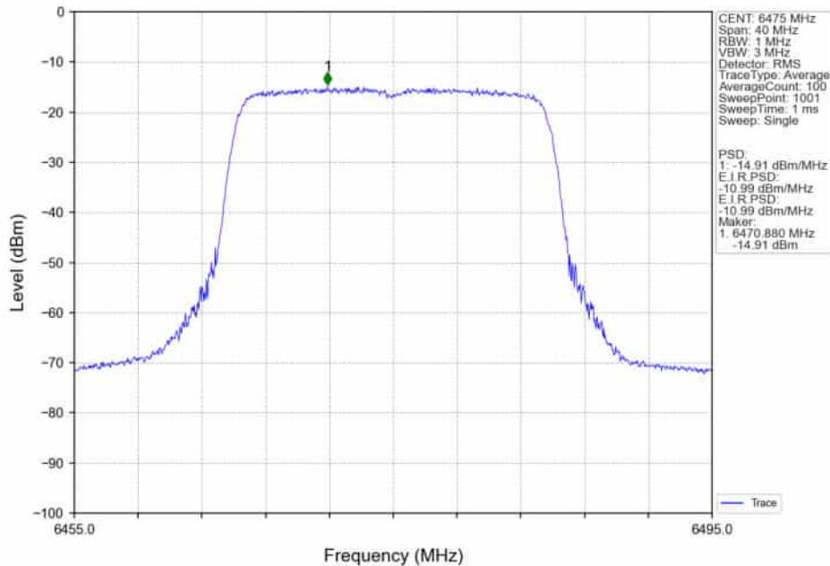
802.11ax(HEW20)_MCH_6475MHz_RU242_Left_MIMO_NTNV
