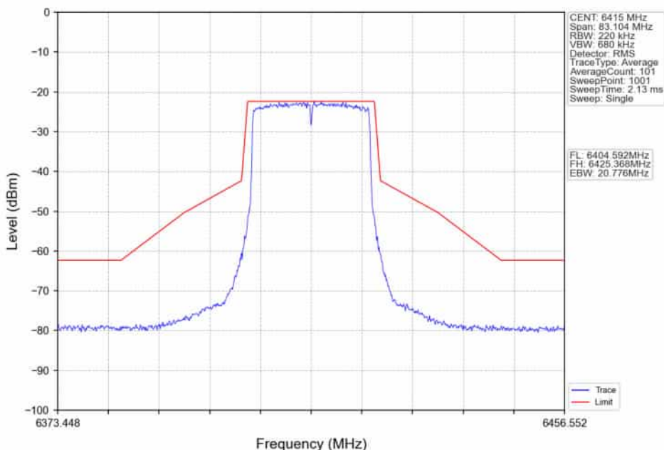
802.11ax(HEW20)_HCH_6415MHz_RU242_Left_Ant2_NTNV
