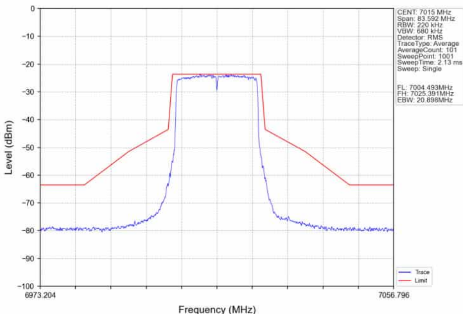
802.11ax(HEW20)_MCH_7015MHz_RU242_Left_Ant2_NTNV
