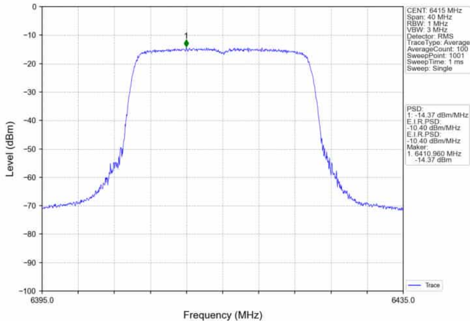
802.11ax(HEW20)_HCH_6415MHz_RU242_Left_Ant2_NTNV
