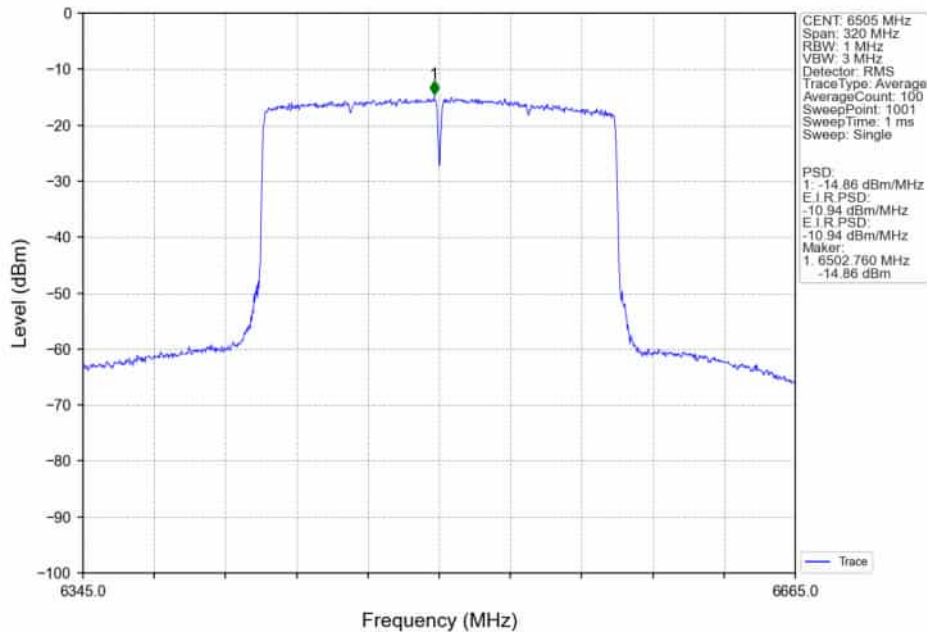
802.11ax(HEW160)_HCH_6505MHz_2xRU996_Left_Ant2_NTNV
