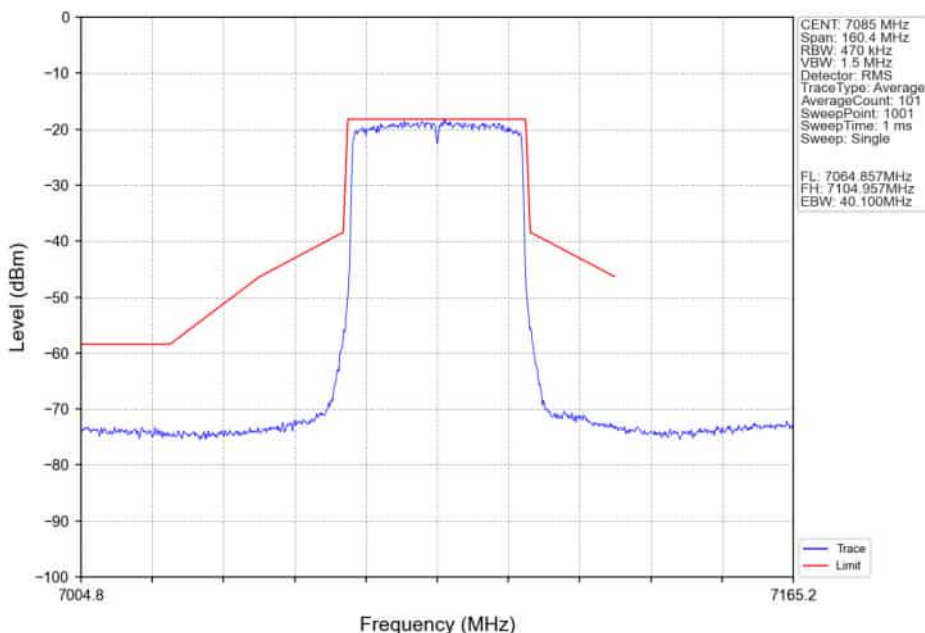
802.11ax(HEW40)_HCH_7085MHz_RU484_Left_Ant2_NTNV
