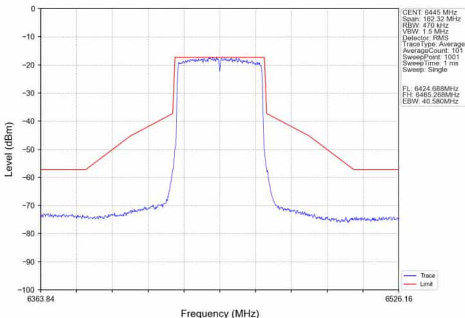
802.11ax(HEW40)_LCH_6445MHz_RU484_Left_Ant2_NTNV
