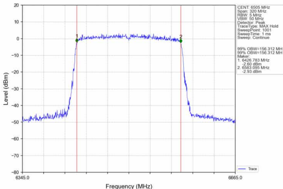
802.11ax(HEW160)_HCH_6505MHz_2xRU996_Left_Ant2_NTNV
