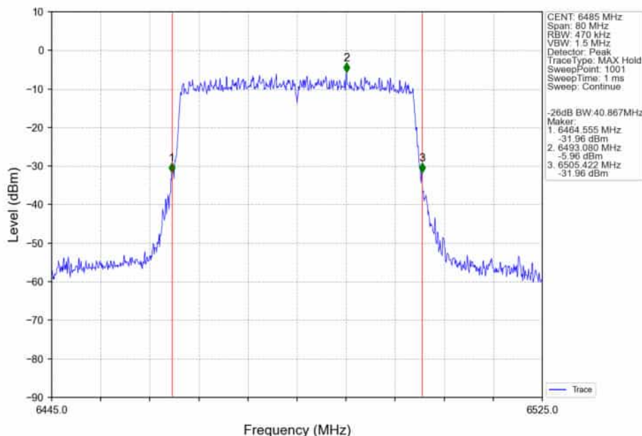
802.11ax(HEW40)_MCH_6485MHz_RU484_Left_Ant2_NTNV
