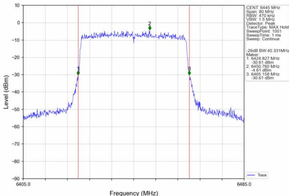
802.11ax(HEW40)_LCH_6445MHz_RU484_Left_Ant2_NTNV
