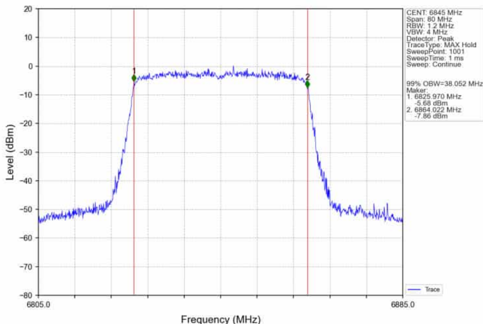
802.11ax(HEW40)_HCH_6845MHz_RU484_Left_Ant2_NTNV
