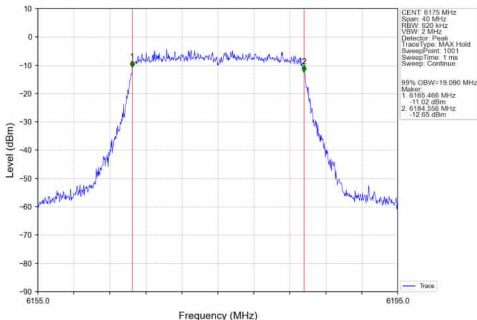
802.11ax(HEW20)_MCH_6175MHz_RU242_Left_Ant2_NTNV
