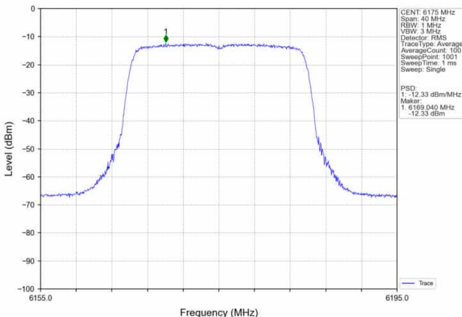
802.11ax(HEW20)_MCH_6175MHz_RU242_Left_MIMO_NTNV
