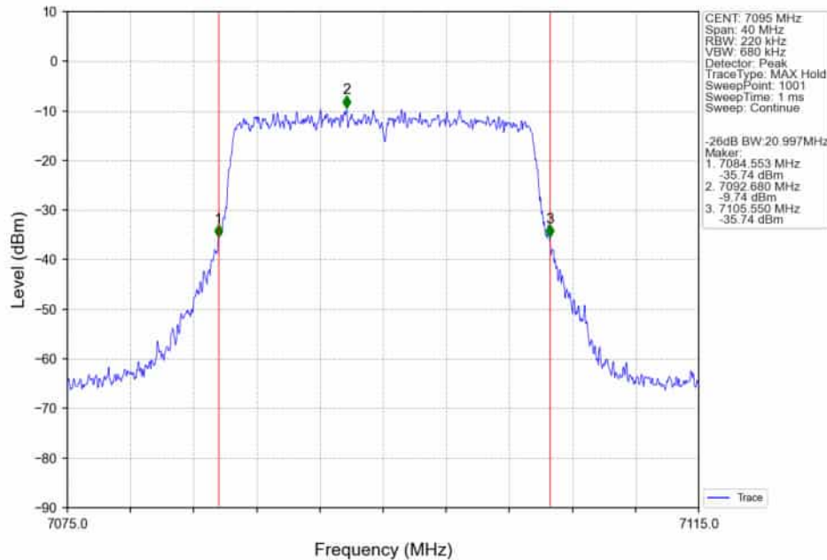
802.11ax(HEW20)_HCH_7095MHz_RU242_Left_Ant2_NTNV
