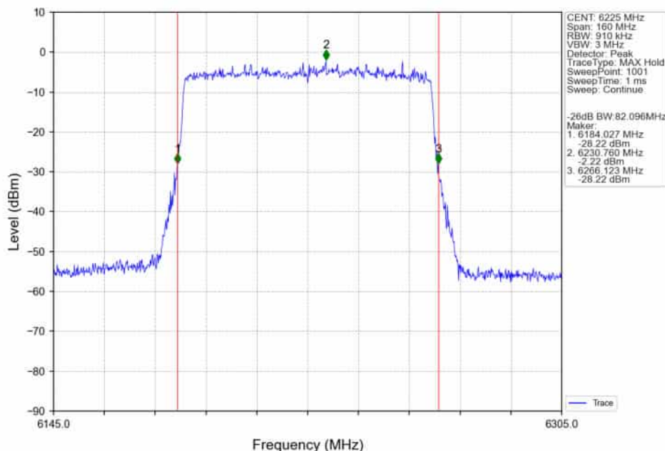
802.11ax(HEW80)_MCH_6225MHz_RU996_Left_Ant2_NTNV
