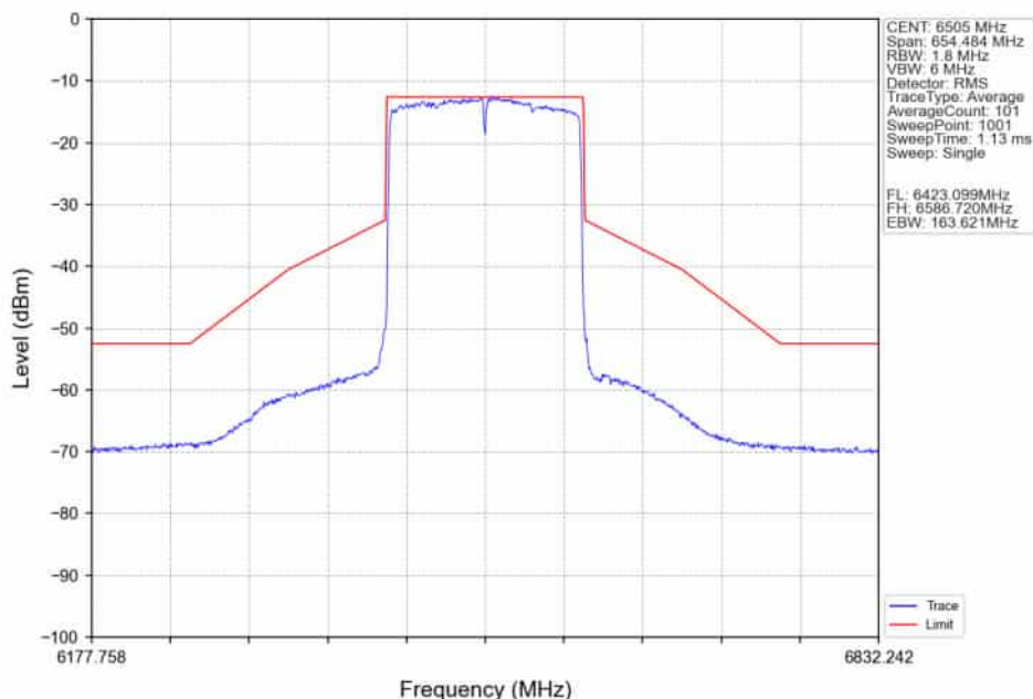
802.11ax(HEW160)_HCH_6505MHz_2xRU996_Left_Ant2_NTNV
