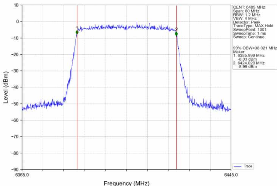
802.11ax(HEW40)_HCH_6405MHz_RU484_Left_Ant2_NTNV
