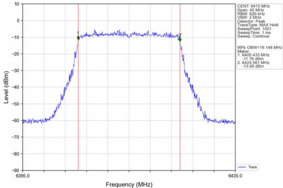
802.11ax(HEW20)_HCH_6415MHz_RU242_Left_Ant2_NTNV
