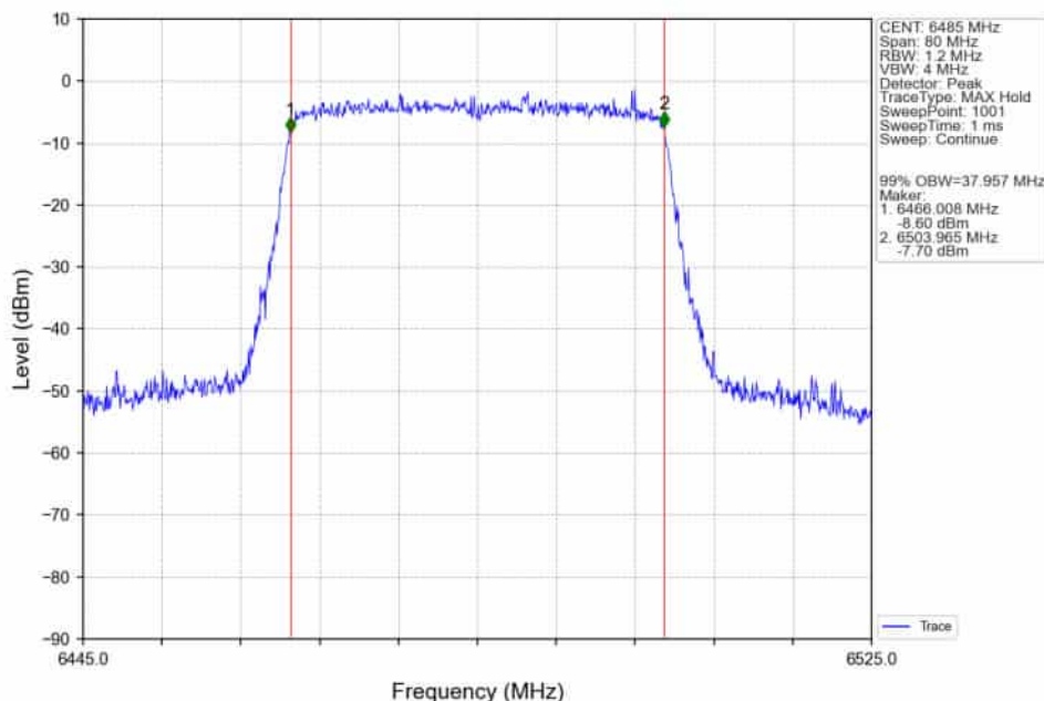
802.11ax(HEW40)_MCH_6485MHz_RU484_Left_Ant2_NTNV
