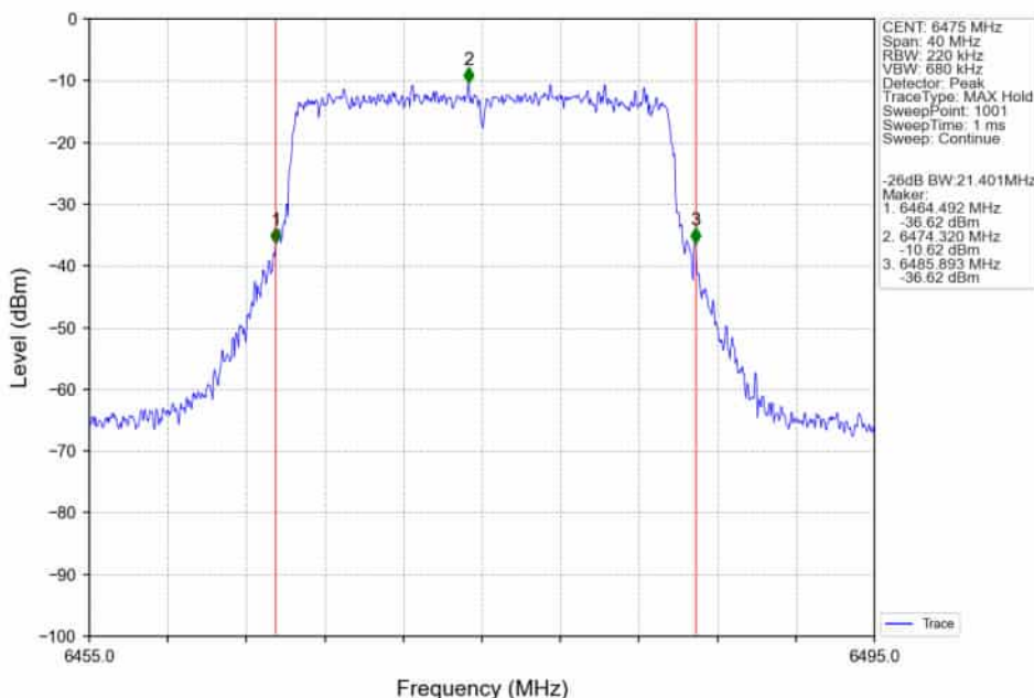
802.11ax(HEW20)_MCH_6475MHz_RU242_Left_Ant2_NTNV
