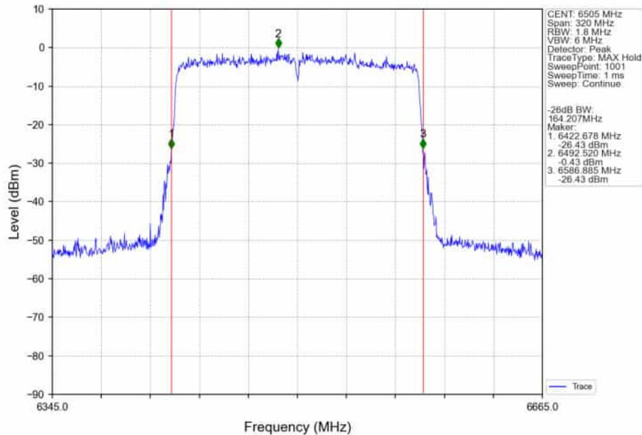
802.11ax(HEW160)_HCH_6505MHz_2xRU996_Left_Ant2_NTNV
