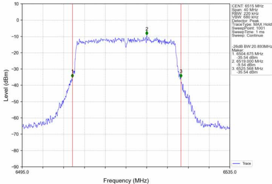
802.11ax(HEW20)_HCH_6515MHz_RU242_Left_Ant2_NTNV
