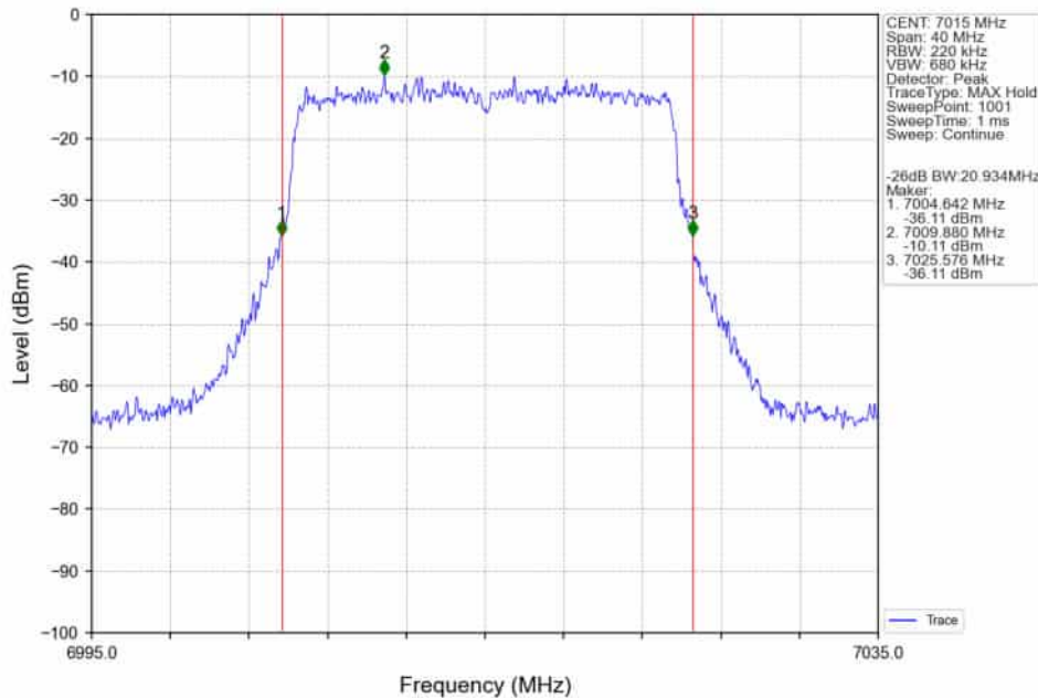
802.11ax(HEW20)_MCH_7015MHz_RU242_Left_Ant2_NTNV
