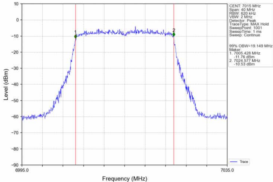
802.11ax(HEW20)_MCH_7015MHz_RU242_Left_Ant2_NTNV
