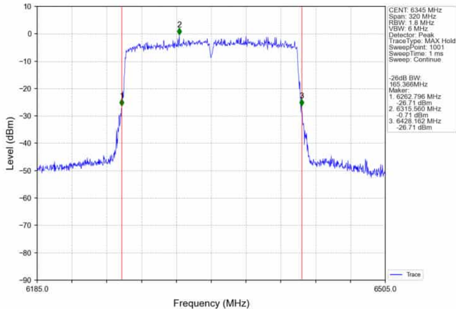
802.11ax(HEW160)_HCH_6345MHz_2xRU996_Left_Ant2_NTNV
