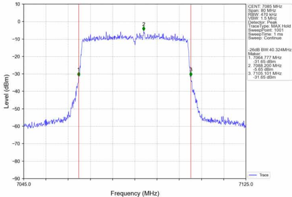
802.11ax(HEW40)_HCH_7085MHz_RU484_Left_Ant2_NTNV
