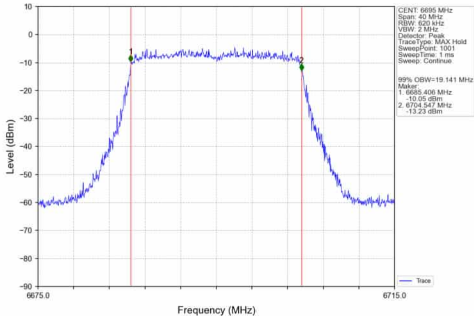
802.11ax(HEW20)_MCH_6695MHz_RU242_Left_Ant2_NTNV
