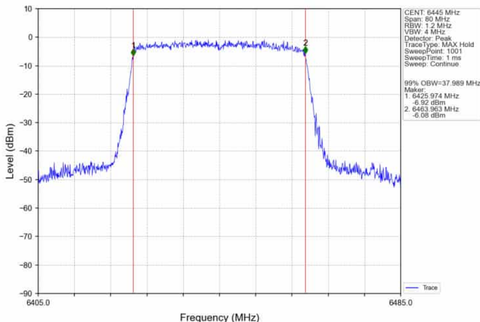
802.11ax(HEW40)_LCH_6445MHz_RU484_Left_Ant2_NTNV
