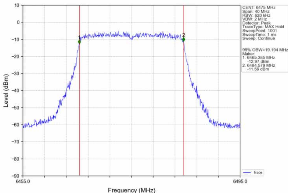
802.11ax(HEW20)_MCH_6475MHz_RU242_Left_Ant2_NTNV
