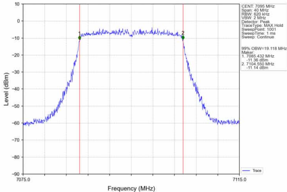
802.11ax(HEW20)_HCH_7095MHz_RU242_Left_Ant2_NTNV
