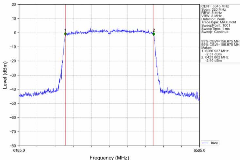
802.11ax(HEW160)_HCH_6345MHz_2xRU996_Left_Ant2_NTNV
