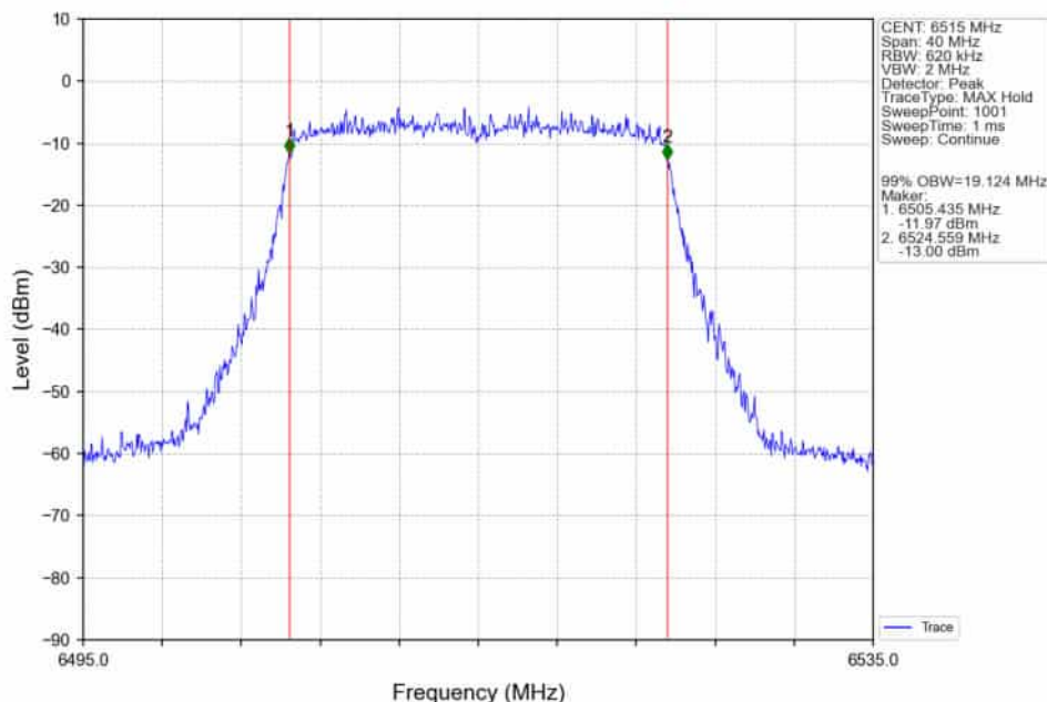
802.11ax(HEW20)_HCH_6515MHz_RU242_Left_Ant2_NTNV
