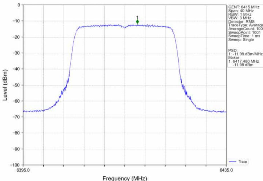
802.11ax(HEW20)_HCH_6415MHz_RU242_Left_Ant2_NTNV
