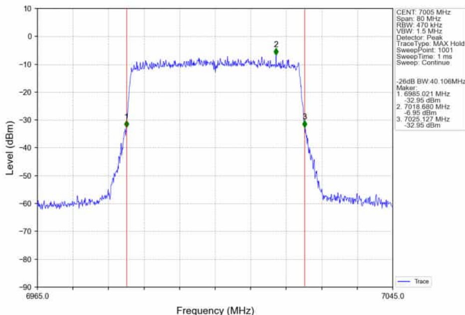
802.11ax(HEW40)_MCH_7005MHz_RU484_Left_Ant2_NTNV
