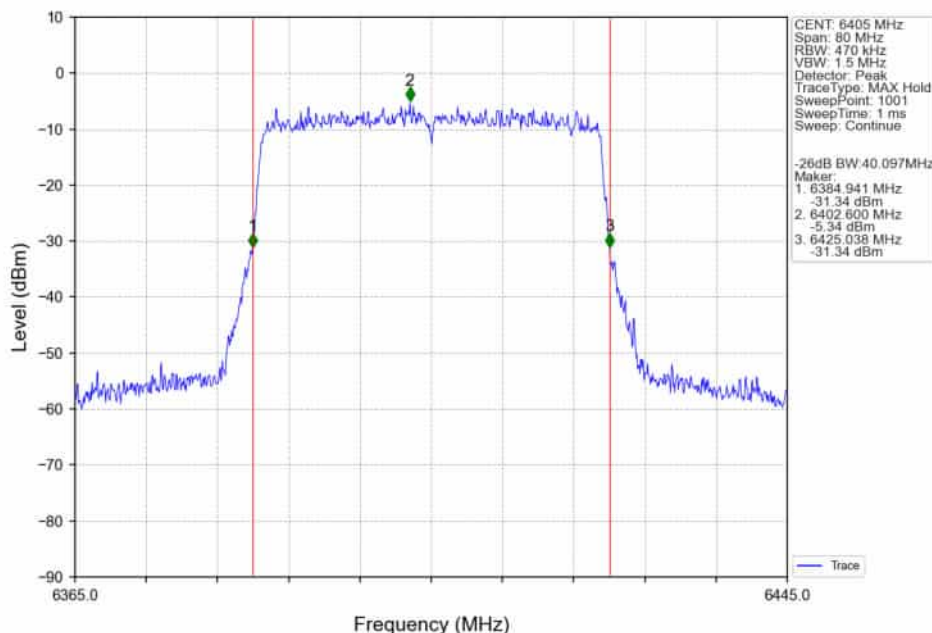
802.11ax(HEW40)_HCH_6405MHz_RU484_Left_Ant2_NTNV
