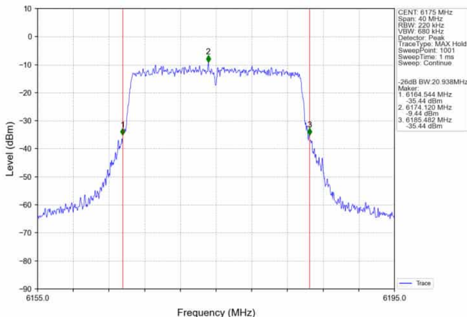
802.11ax(HEW20)_MCH_6175MHz_RU242_Left_Ant2_NTNV
