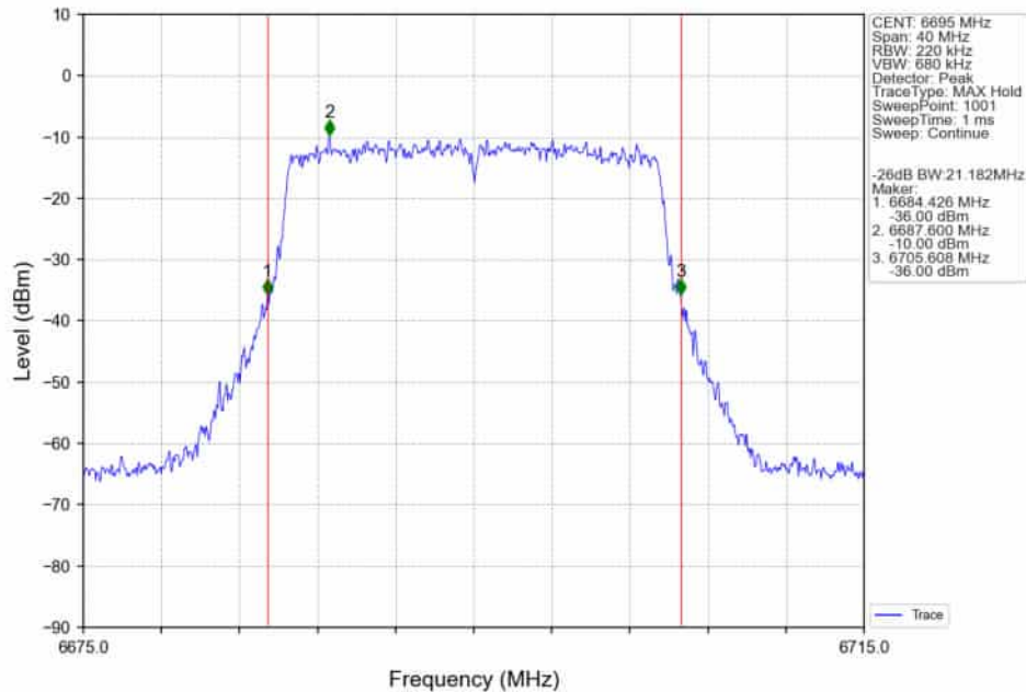
802.11ax(HEW20)_MCH_6695MHz_RU242_Left_Ant2_NTNV
