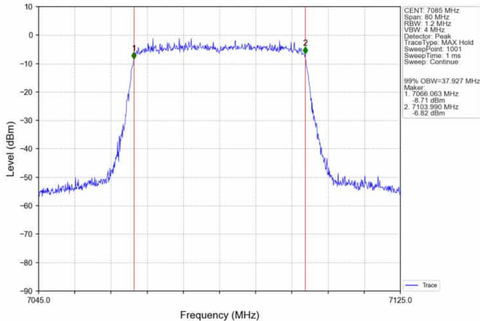
802.11ax(HEW40)_HCH_7085MHz_RU484_Left_Ant2_NTNV
