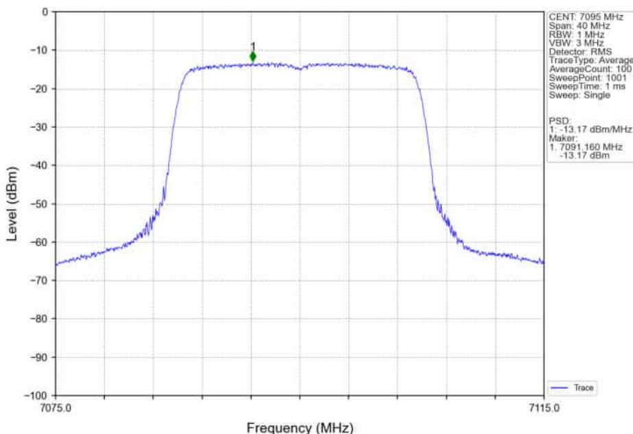
802.11ax(HEW20)_HCH_7095MHz_RU242_Left_Ant2_NTNV
