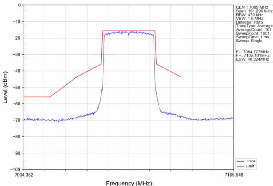
802.11ax(HEW40)_HCH_7085MHz_RU484_Left_Ant2_NTNV
