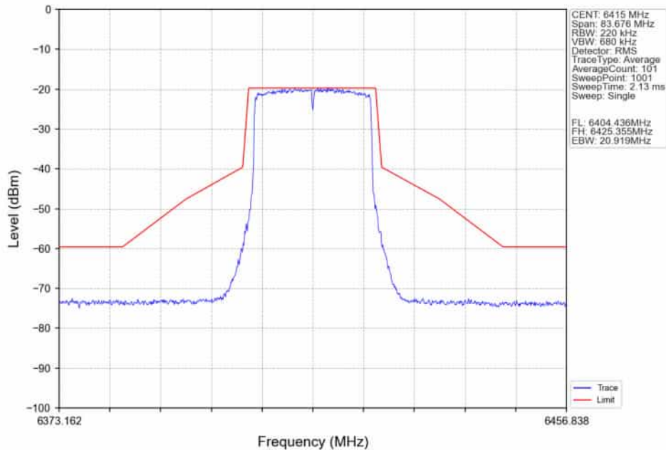
802.11ax(HEW20)_HCH_6415MHz_RU242_Left_Ant2_NTNV
