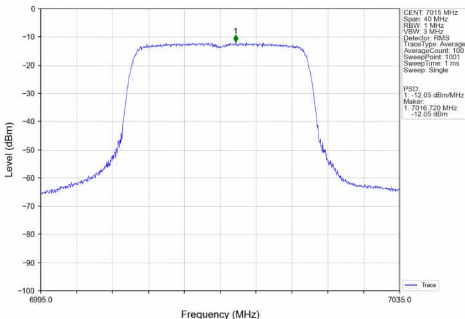
802.11ax(HEW20)_MCH_7015MHz_RU242_Left_MIMO_NTNV
