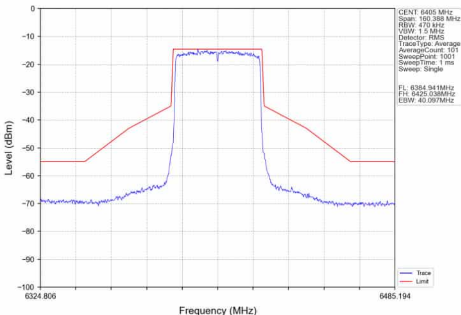
802.11ax(HEW40)_HCH_6405MHz_RU484_Left_Ant2_NTNV
