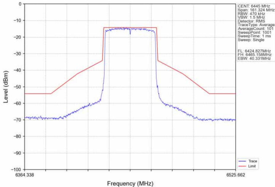
802.11ax(HEW40)_LCH_6445MHz_RU484_Left_Ant2_NTNV
