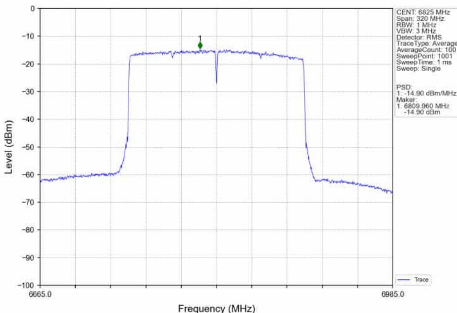
802.11ax(HEW160)_HCH_6825MHz_2xRU996_Left_MIMO_NTNV
