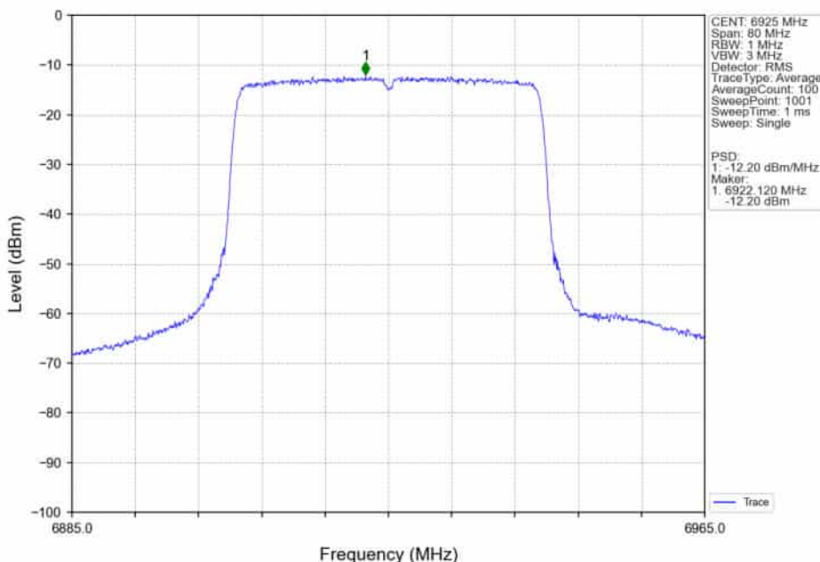
802.11ax(HEW40)_LCH_6925MHz_RU484_Left_MIMO_NTNV
