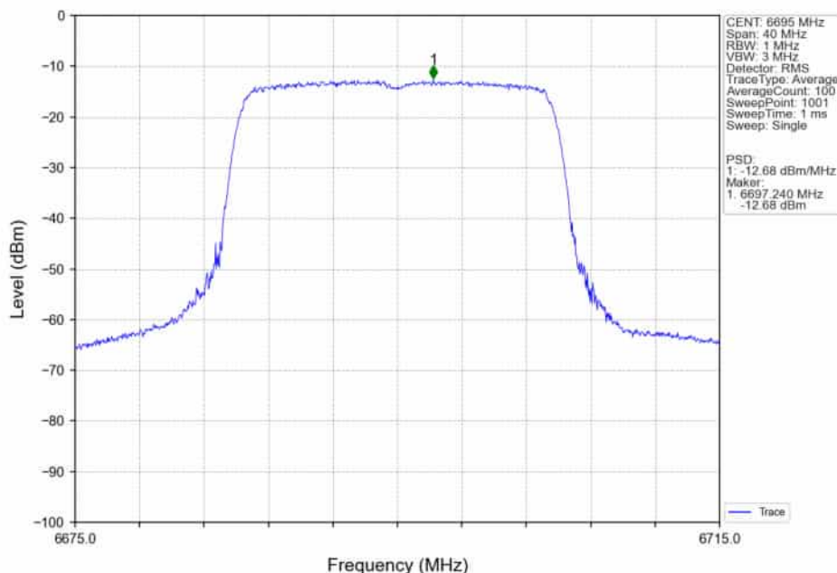
802.11ax(HEW20)_MCH_6695MHz_RU242_Left_MIMO_NTNV
