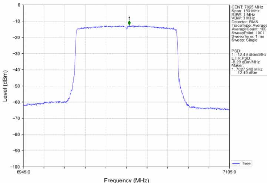
802.11ax(HEW80)_HCH_7025MHz_RU996_Left_MIMO_NTNV
