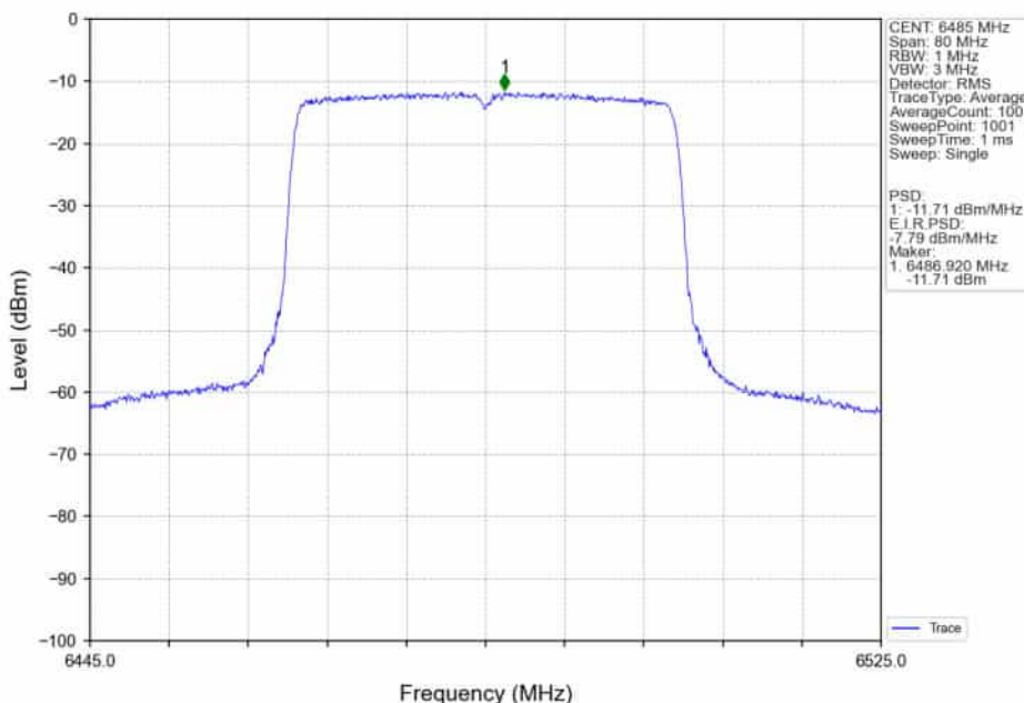
802.11ax(HEW40)_MCH_6485MHz_RU484_Left_Ant2_NTNV
