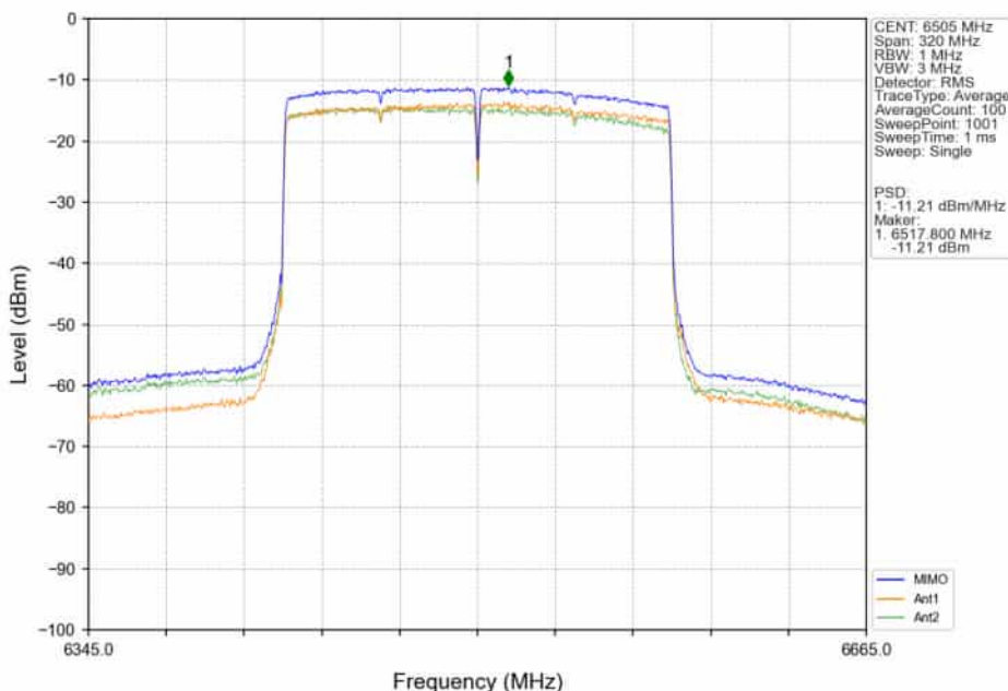
802.11ax(HEW160)_HCH_6505MHz_2xRU996_Left_MIMO_NTNV
