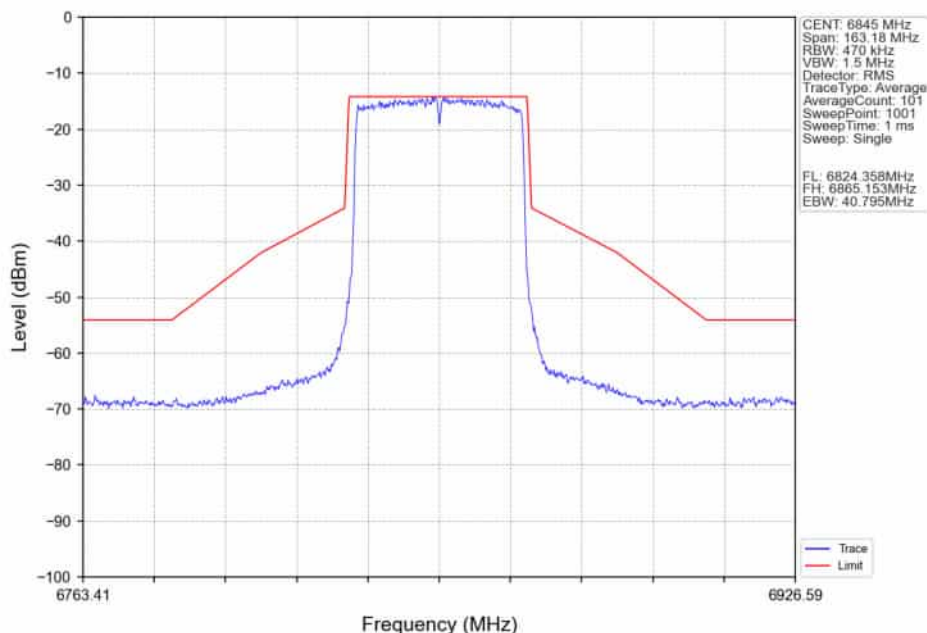
802.11ax(HEW40)_HCH_6845MHz_RU484_Left_Ant2_NTNV
