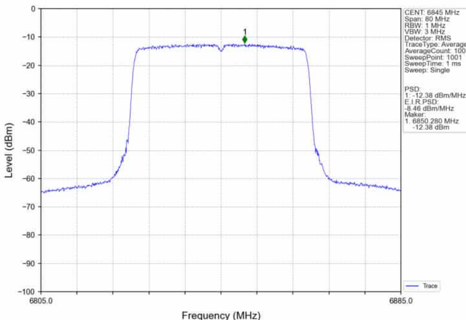
802.11ax(HEW40)_HCH_6845MHz_RU484_Left_MIMO_NTNV
