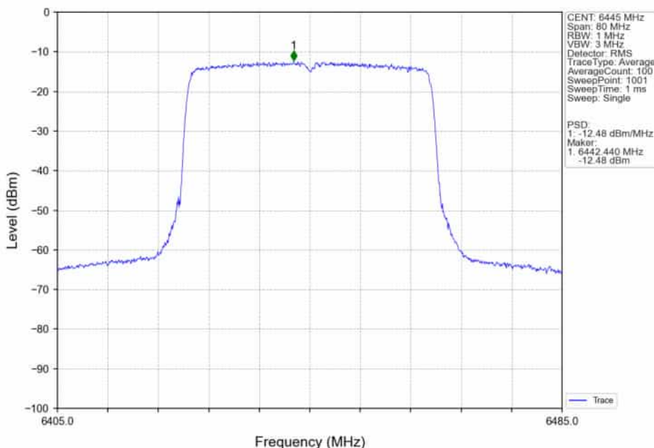
802.11ax(HEW40)_LCH_6445MHz_RU484_Left_MIMO_NTNV
