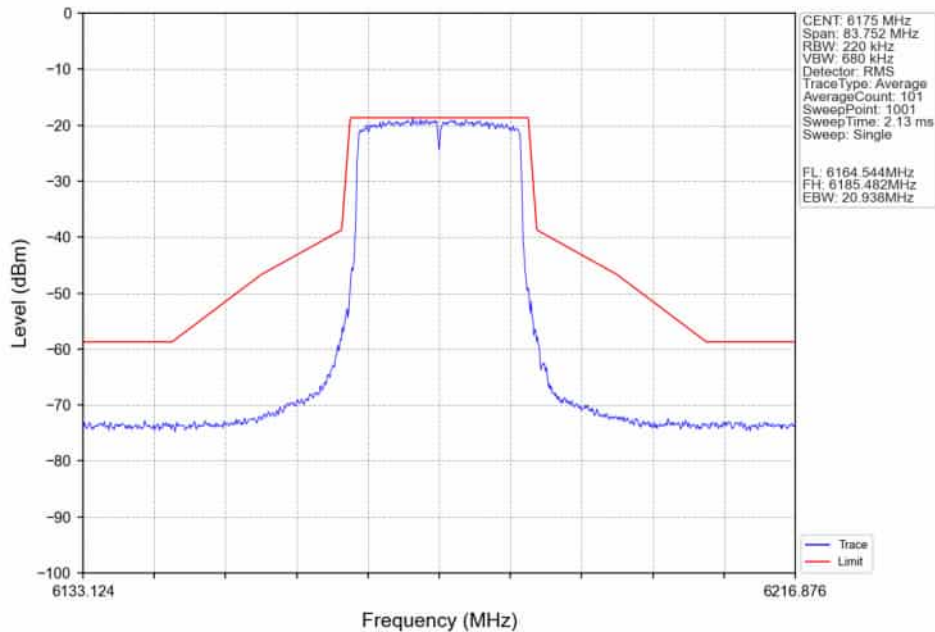
802.11ax(HEW20)_MCH_6175MHz_RU242_Left_Ant2_NTNV
