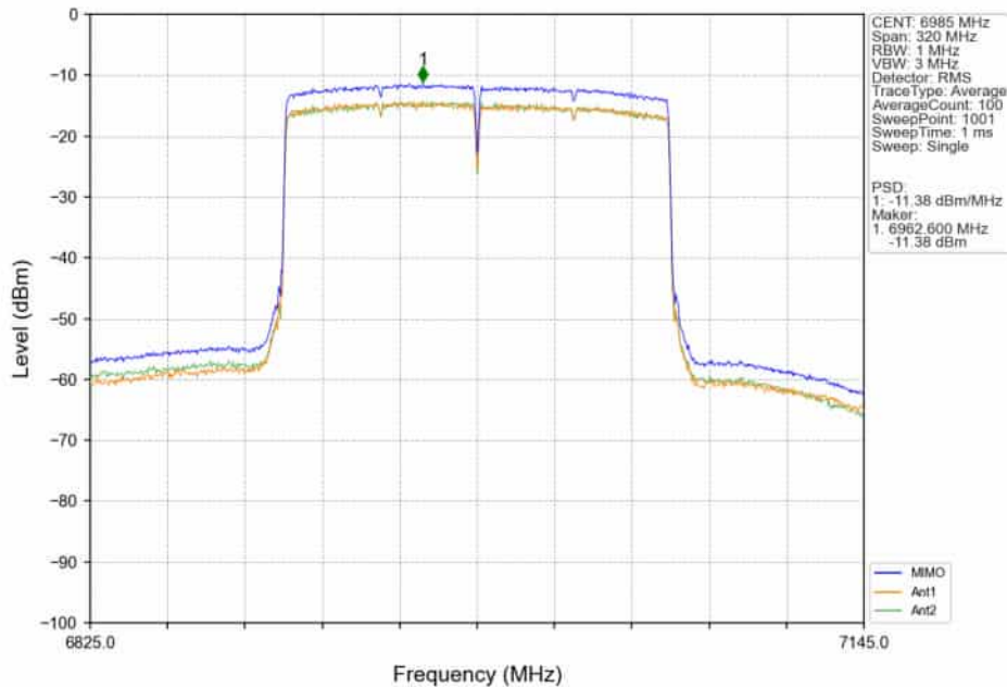
802.11ax(HEW160)_MCH_6985MHz_2xRU996_Left_MIMO_NTNV
