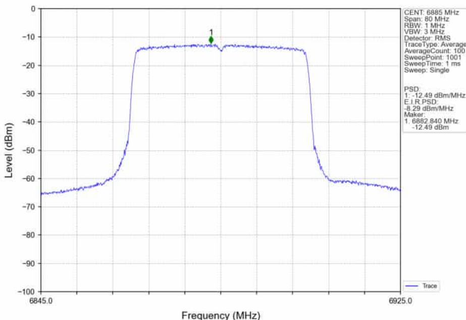
802.11ax(HEW40)_HCH_6885MHz_RU484_Left_MIMO_NTNV
