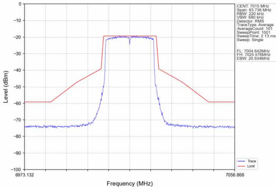
802.11ax(HEW20)_MCH_7015MHz_RU242_Left_Ant2_NTNV
