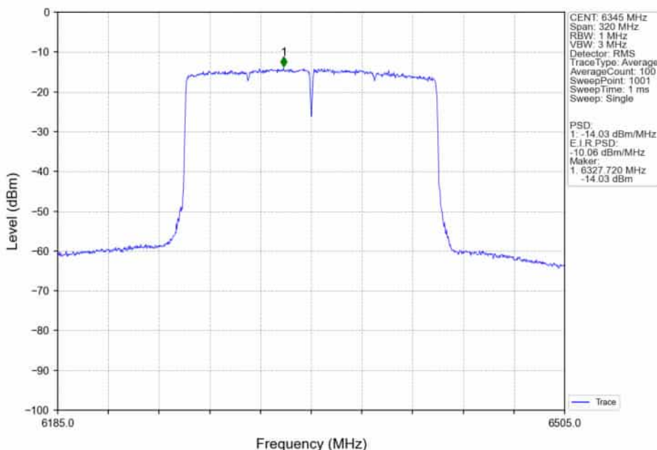
802.11ax(HEW160)_HCH_6345MHz_2xRU996_Left_MIMO_NTNV
