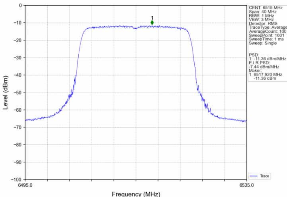
802.11ax(HEW20)_HCH_6515MHz_RU242_Left_Ant2_NTNV
