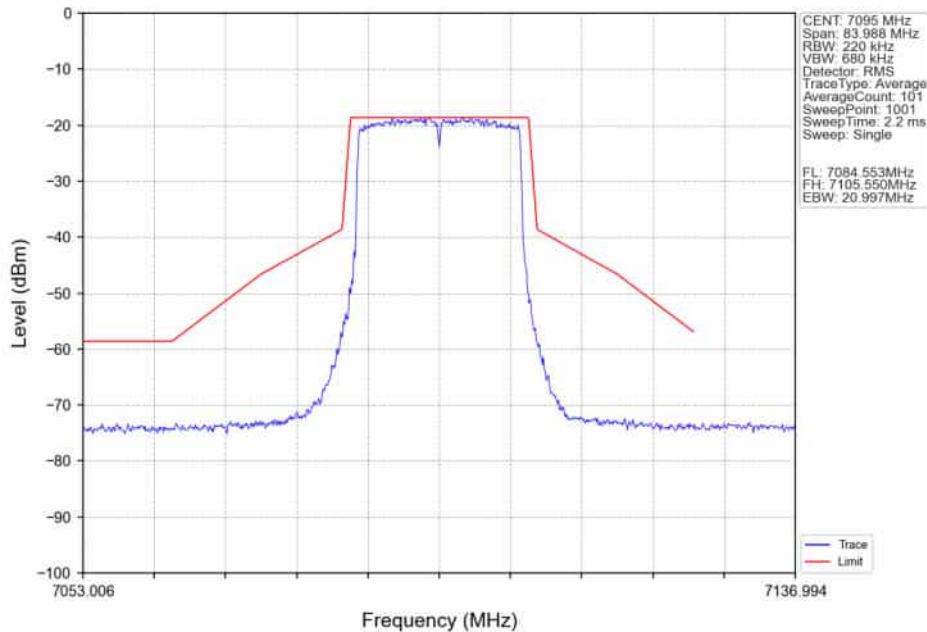
802.11ax(HEW20)_HCH_7095MHz_RU242_Left_Ant2_NTNV
