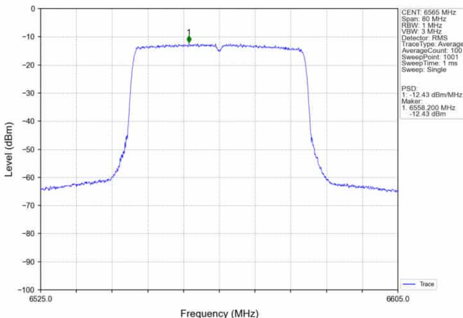
802.11ax(HEW40)_LCH_6565MHz_RU484_Left_MIMO_NTNV
