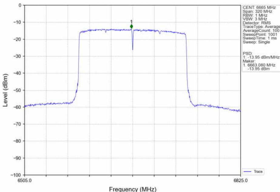
802.11ax(HEW160)_MCH_6665MHz_2xRU996_Left_MIMO_NTNV
