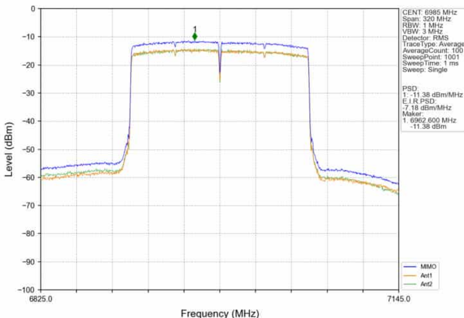
802.11ax(HEW160)_MCH_6985MHz_2xRU996_Left_MIMO_NTNV
