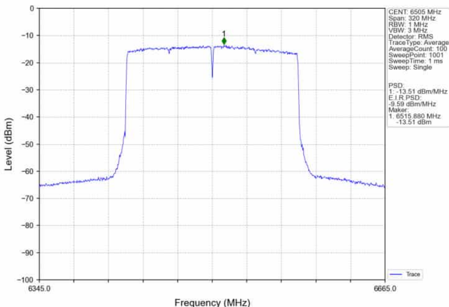
802.11ax(HEW160)_HCH_6505MHz_2xRU996_Left_Ant2_NTNV
