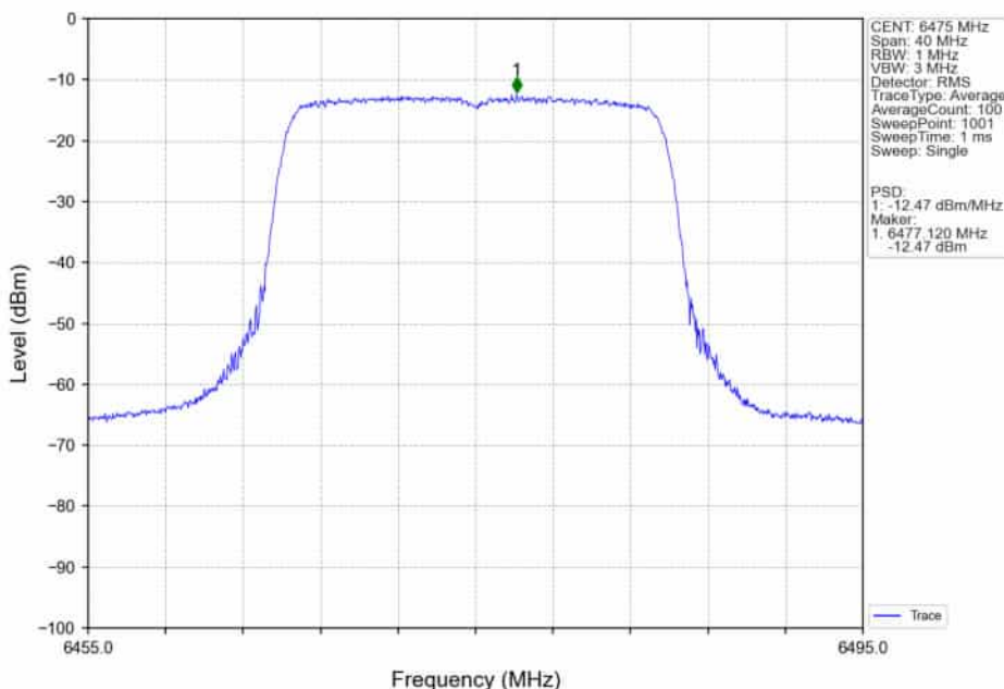
802.11ax(HEW20)_MCH_6475MHz_RU242_Left_MIMO_NTNV
