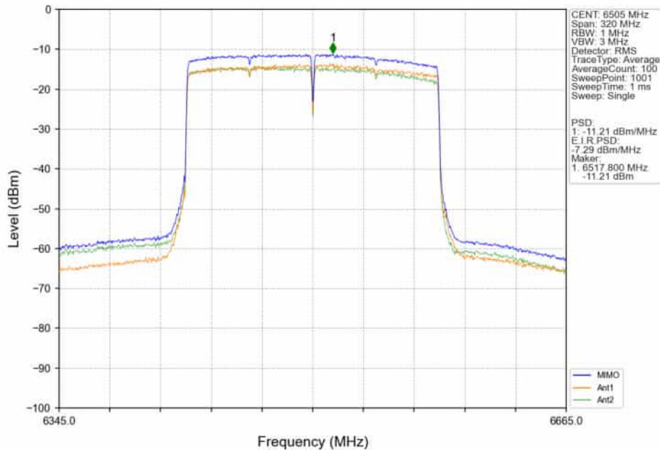
802.11ax(HEW160)_HCH_6505MHz_2xRU996_Left_MIMO_NTNV
