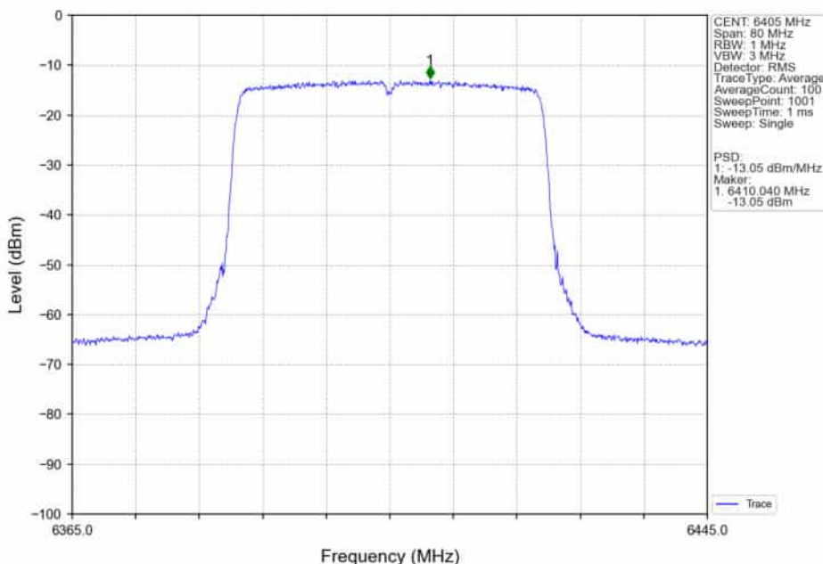
802.11ax(HEW40)_HCH_6405MHz_RU484_Left_MIMO_NTNV
