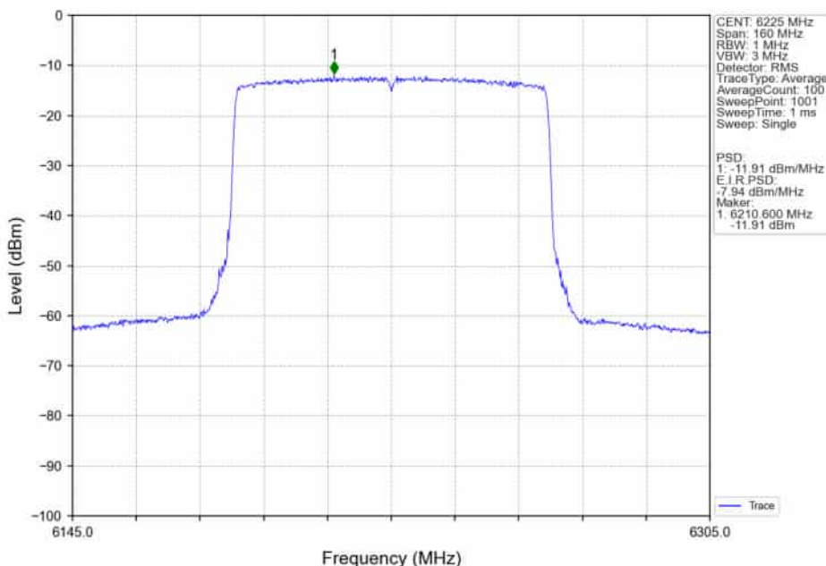
802.11ax(HEW80)_MCH_6225MHz_RU996_Left_MIMO_NTNV
