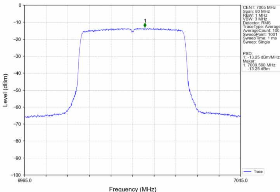
802.11ax(HEW40)_MCH_7005MHz_RU484_Left_Ant2_NTNV
