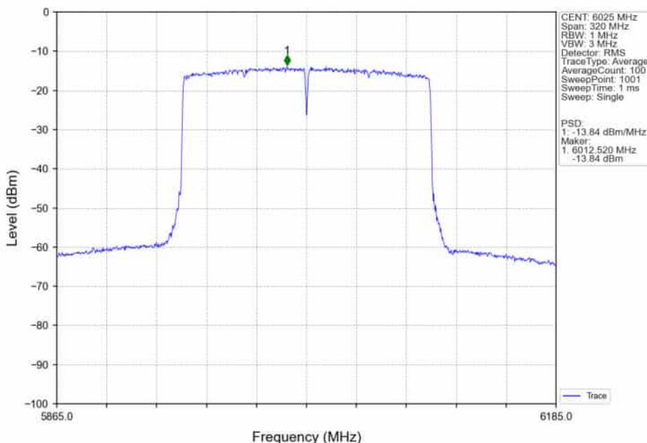
802.11ax(HEW160)_LCH_6025MHz_2xRU996_Left_MIMO_NTNV
