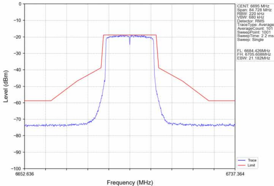
802.11ax(HEW20)_MCH_6695MHz_RU242_Left_Ant2_NTNV
