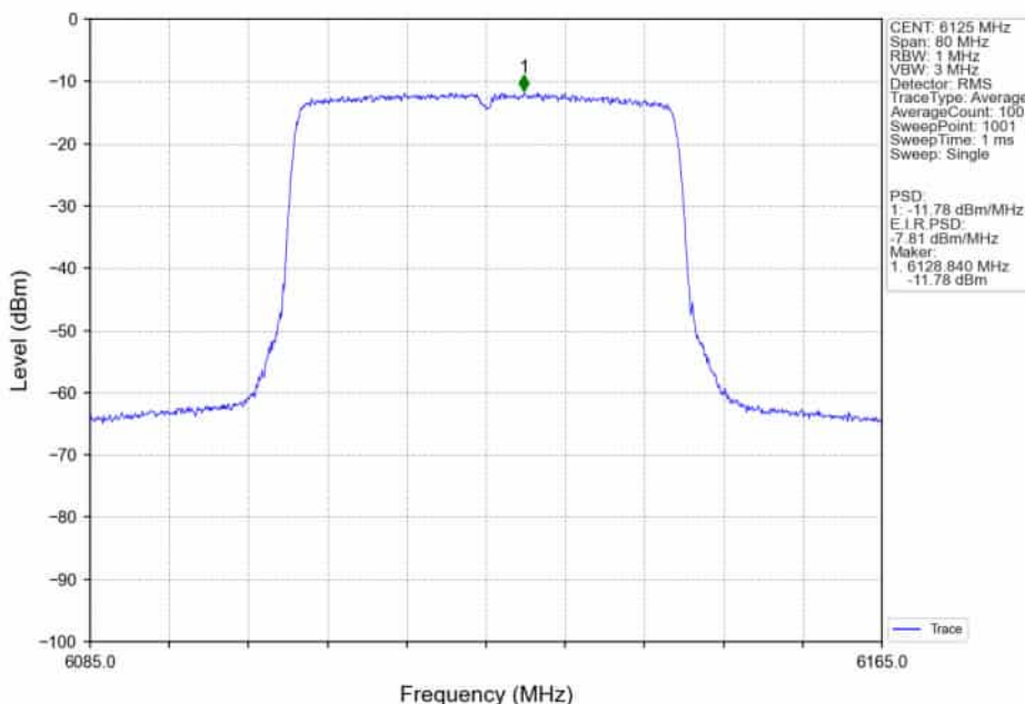
802.11ax(HEW40)_LCH_6125MHz_RU484_Left_MIMO_NTNV
