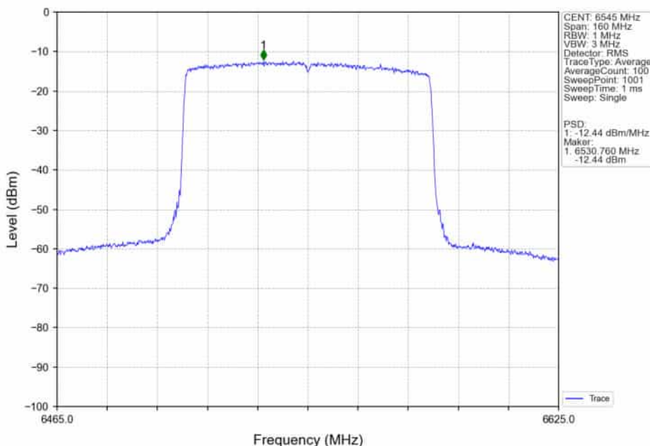
802.11ax(HEW80)_HCH_6545MHz_RU996_Left_MIMO_NTNV
