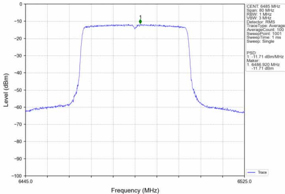
802.11ax(HEW40)_MCH_6485MHz_RU484_Left_Ant2_NTNV
