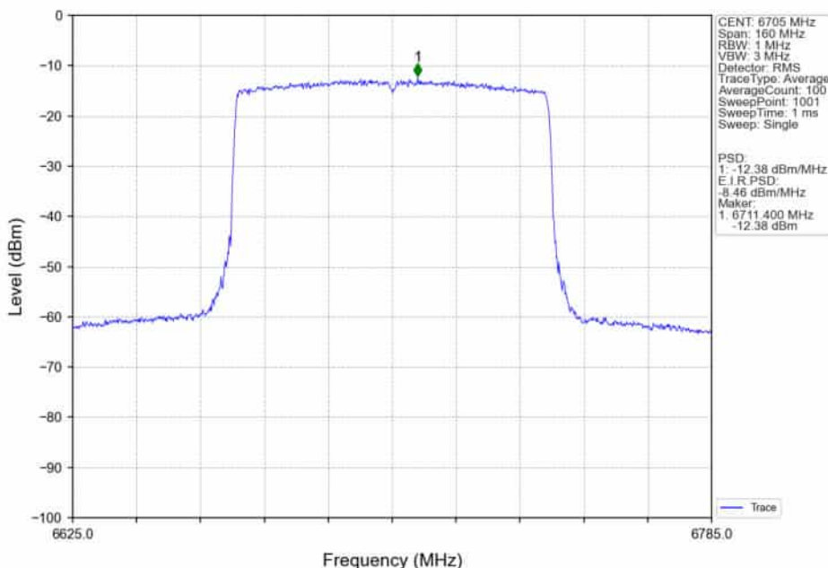
802.11ax(HEW80)_MCH_6705MHz_RU996_Left_MIMO_NTNV
