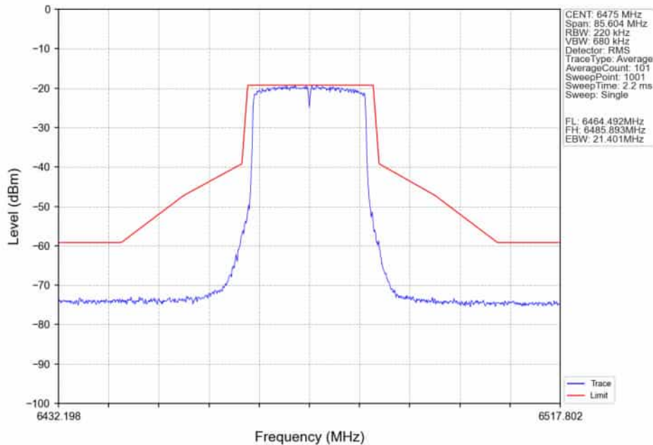
802.11ax(HEW20)_MCH_6475MHz_RU242_Left_Ant2_NTNV
