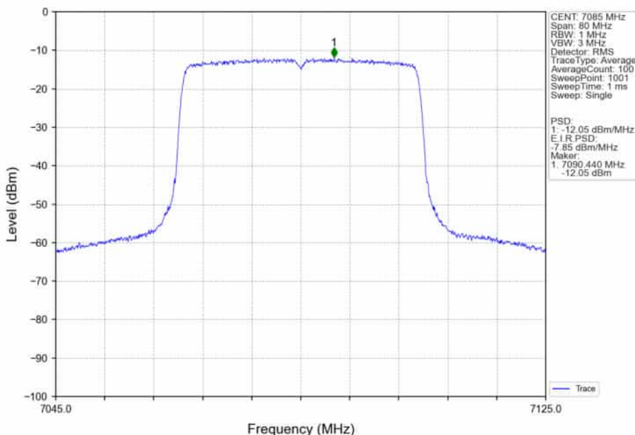
802.11ax(HEW40)_HCH_7085MHz_RU484_Left_MIMO_NTNV
