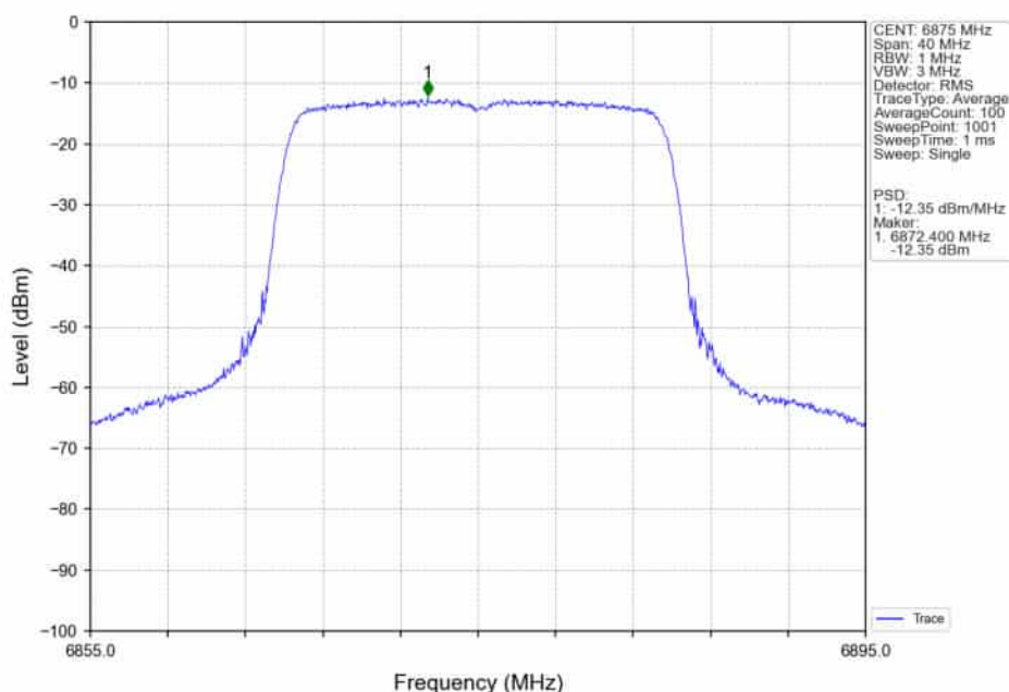
802.11ax(HEW20)_HCH_6875MHz_RU242_Left_Ant2_NTNV
