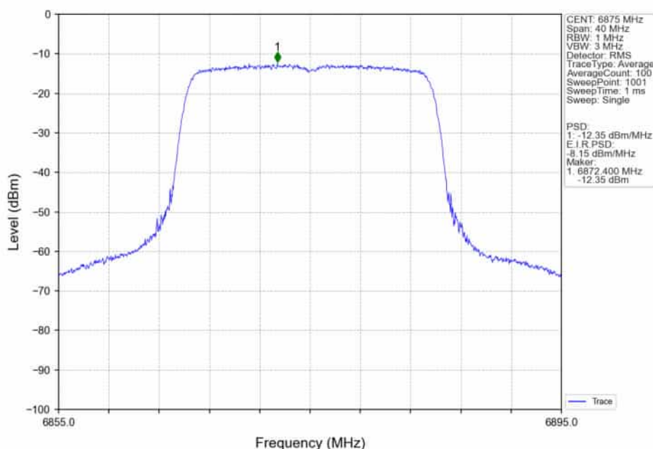
802.11ax(HEW20)_HCH_6875MHz_RU242_Left_Ant2_NTNV
