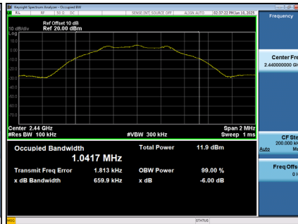
CH19 6 dB Bandwidth
