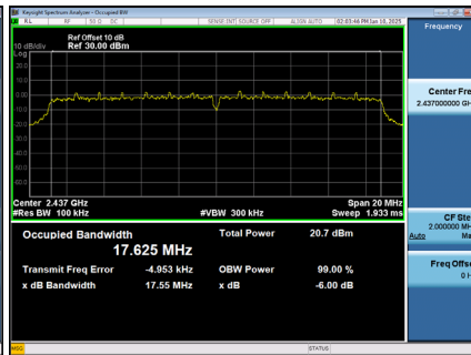
6 dB Bandwidth
