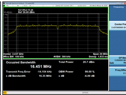
99 % Occupied Bandwidth
