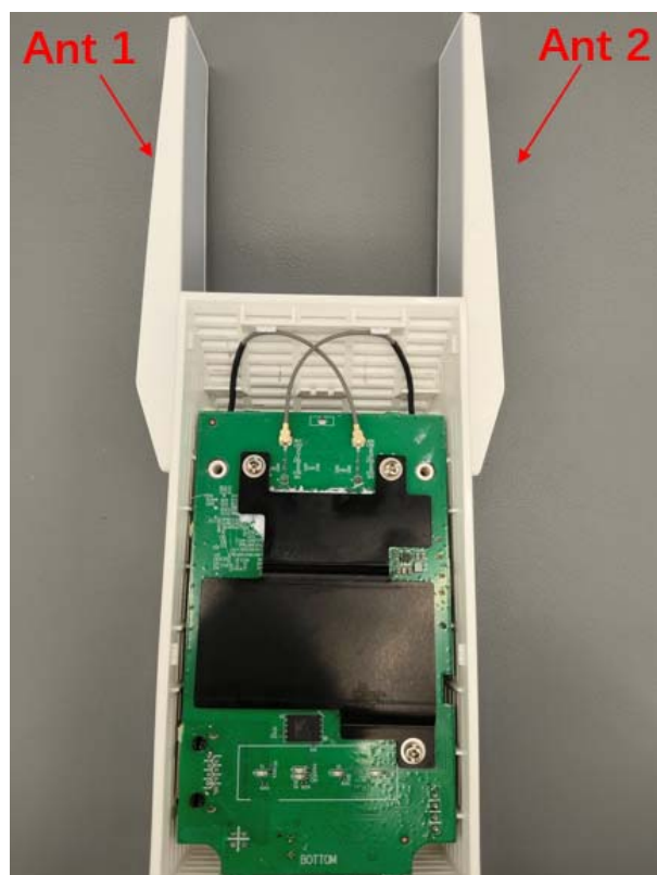
Figure 1-1 Locations of Antennas
