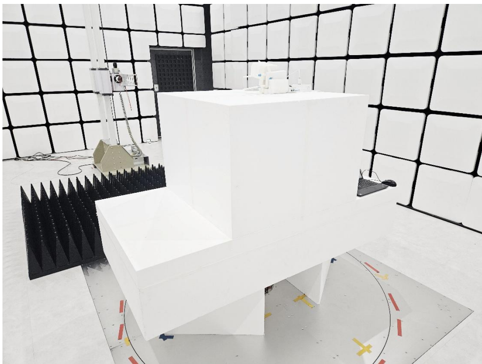
Description: Radiated Emission Test Setup for above 1GHz_2.4G
