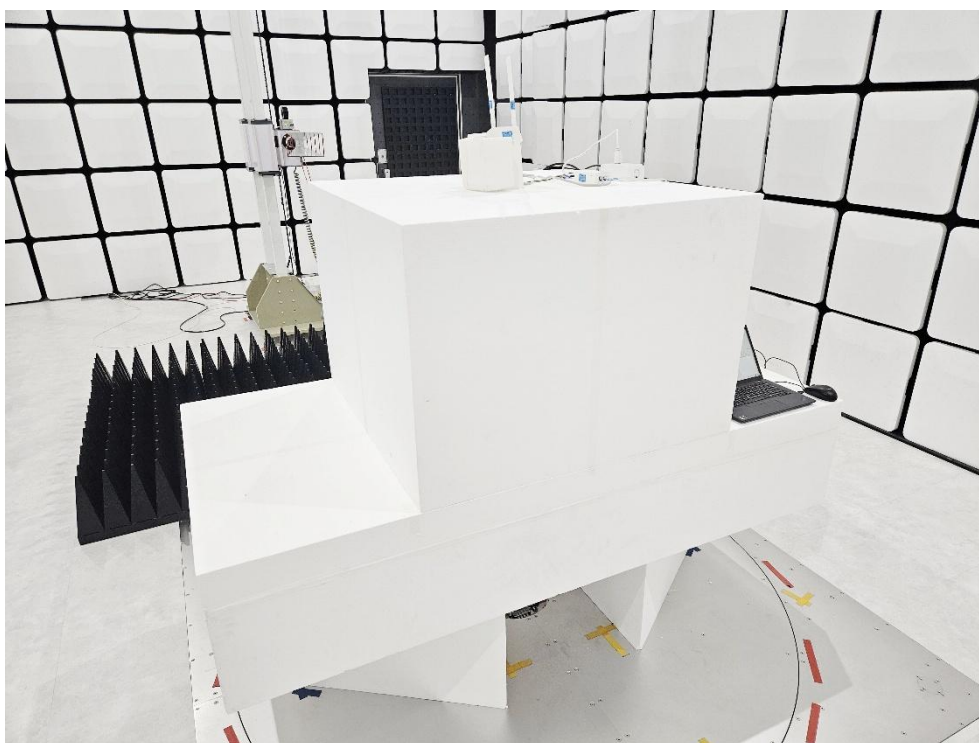
Description: Radiated Emission Test Setup for above 1GHz_5G
