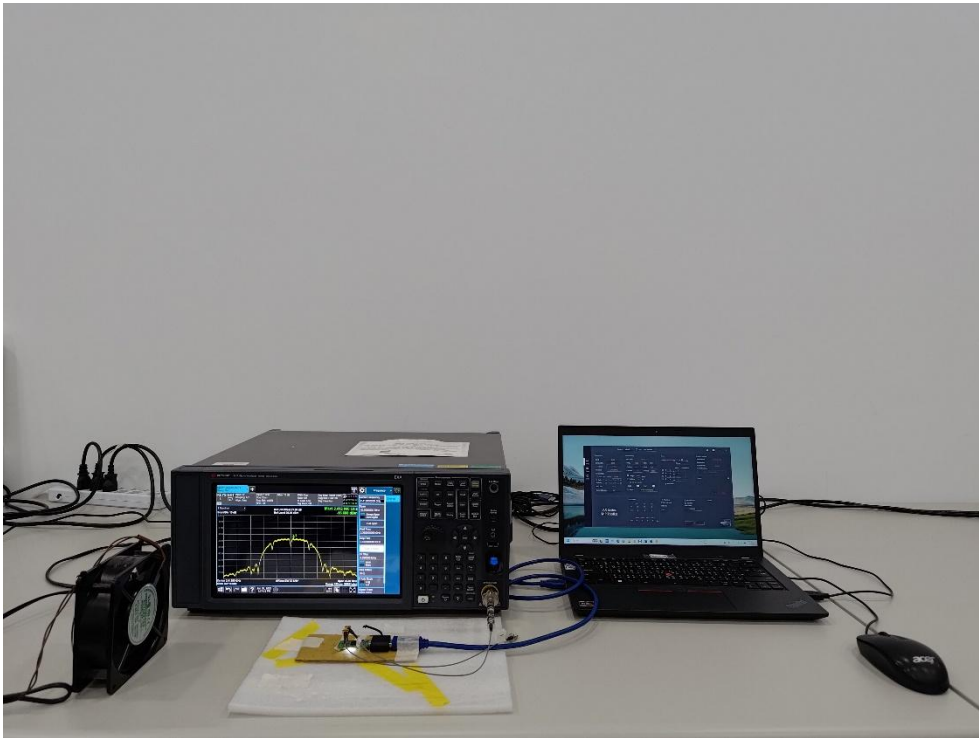
Description: Adaptivity Test Setup
