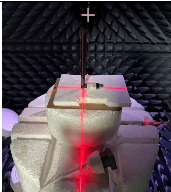
Figure 3-4 Antennas measurement diagram
