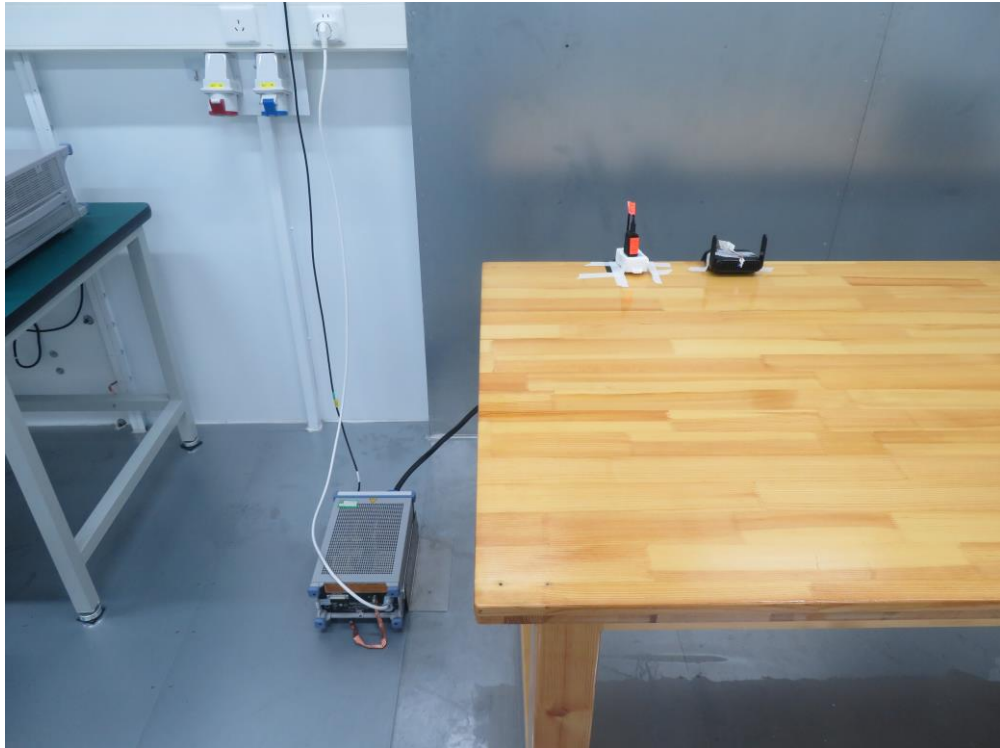
Description: Side View of Conducted Test Setup
