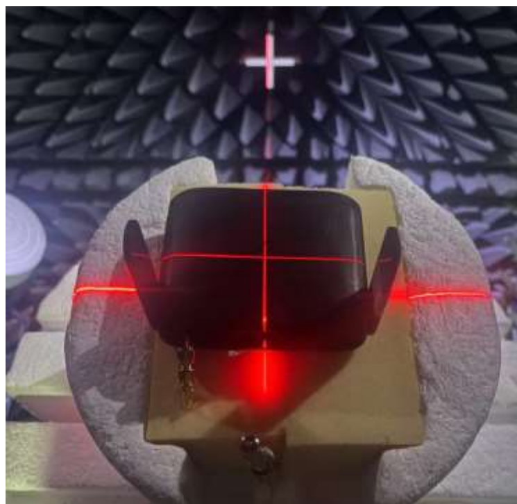
Figure 3-4 Antennas measurement diagram
