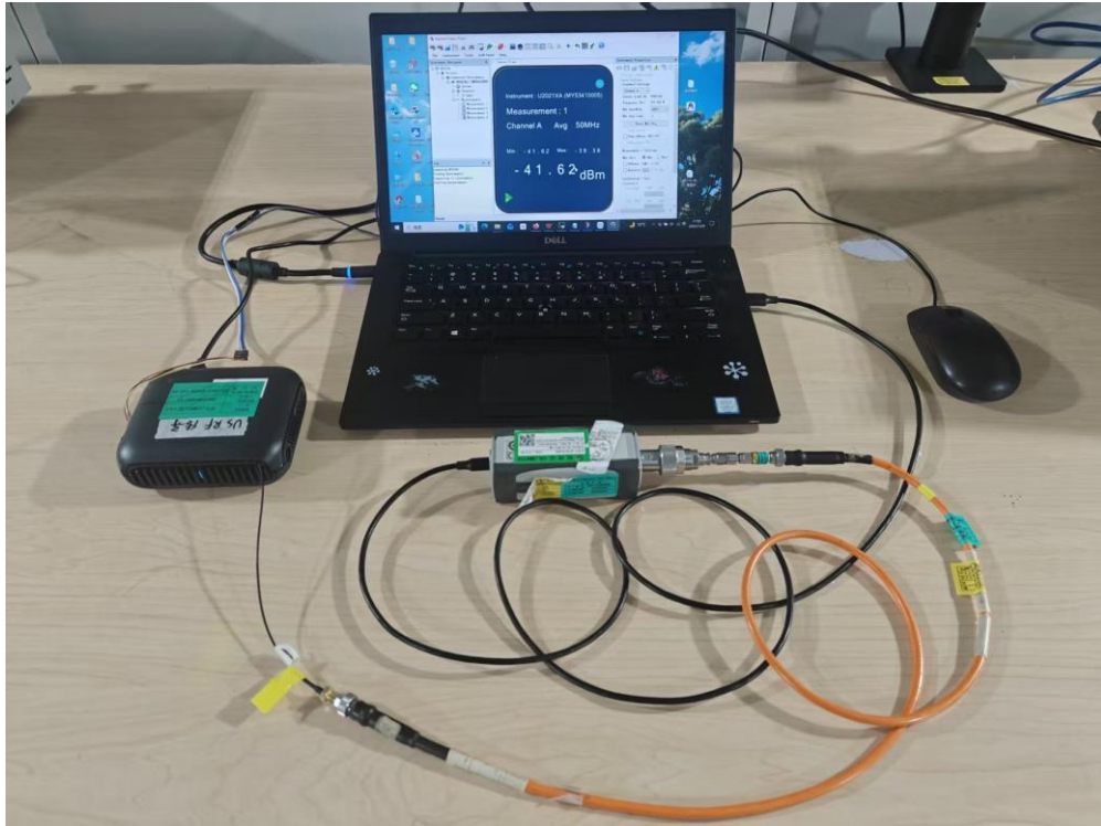
Description: DFS Test Setup (SIP-TR1)
