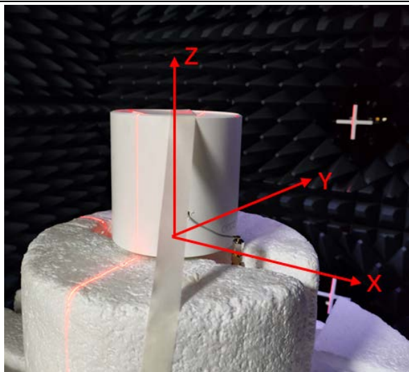
Figure 3-4 Antennas measurement diagram
