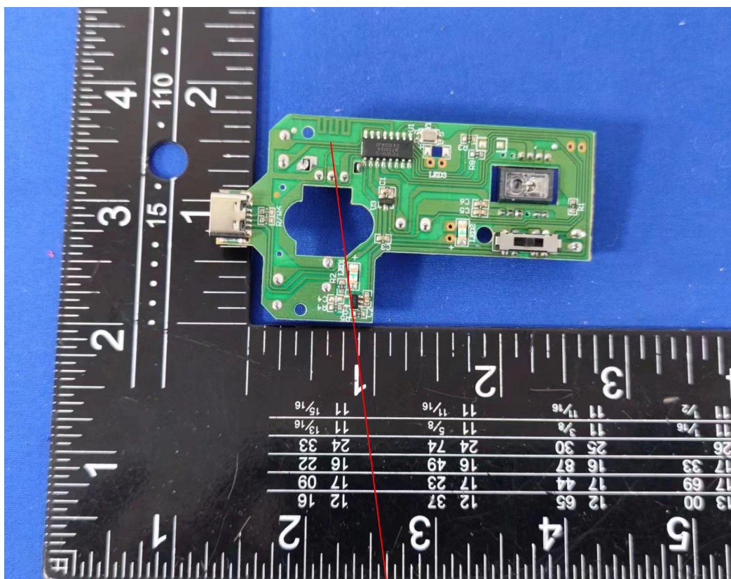
PCB ANTENNA
