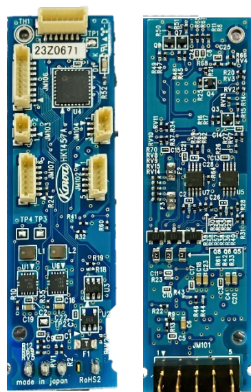
HK1457A PCB Front Back
