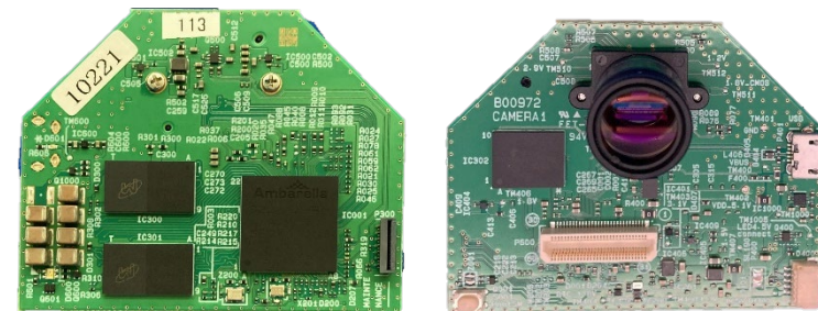
PCB Camera1 Front Back
