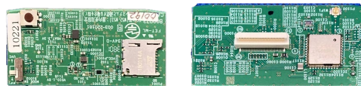
PCB Camera2 = Wireless Module Front Back
