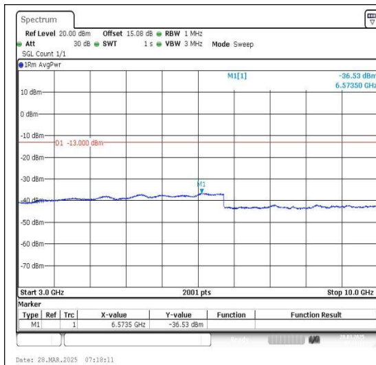
Band12_1.4MHz_QPSK_23017_1RB#0_3000~10000_3000~10000
