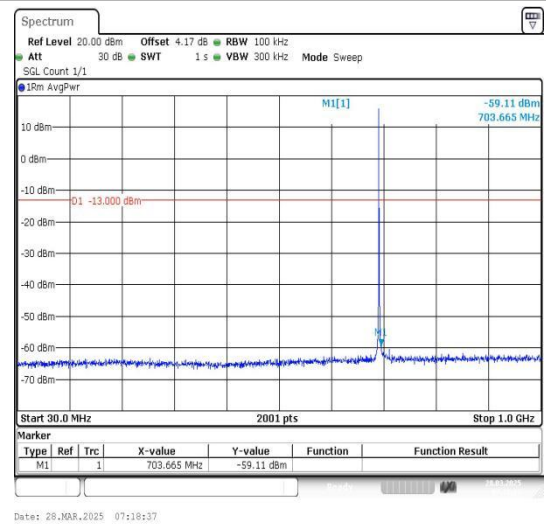
Band12_1.4MHz_16QAM_23017_1RB#0_30~100_30~1000
