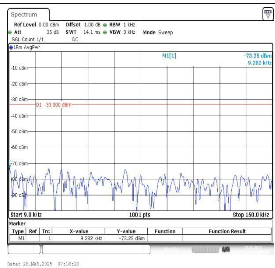
Band12_1.4MHz_16QAM_23017_1RB#0_0.009~0.15_0.009~0.15
