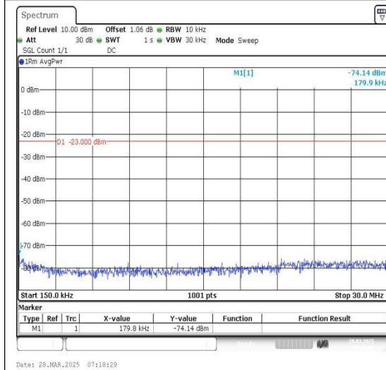
Band12_1.4MHz_16QAM_23017_1RB#0_0.15~30_0.15~30
