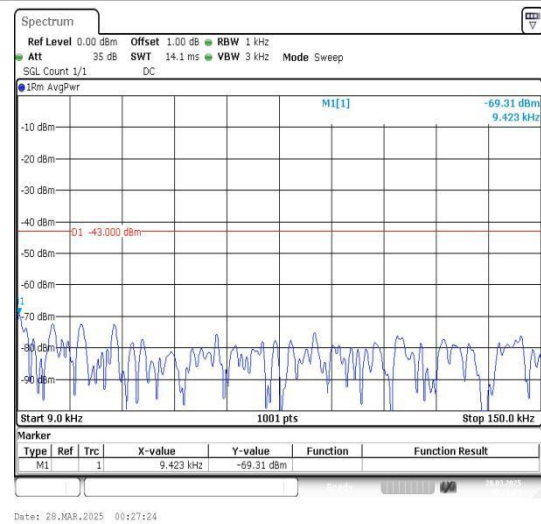
Band4_3MHz_16QAM_19965_1RB#0_0.009~0.15 _0.009~0.15
