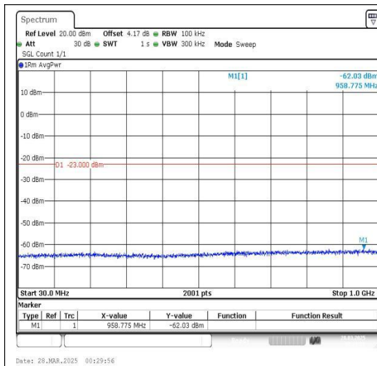
Band4_3MHz_QPSK_20385_1RB#0_30~1000_3 0~1000
