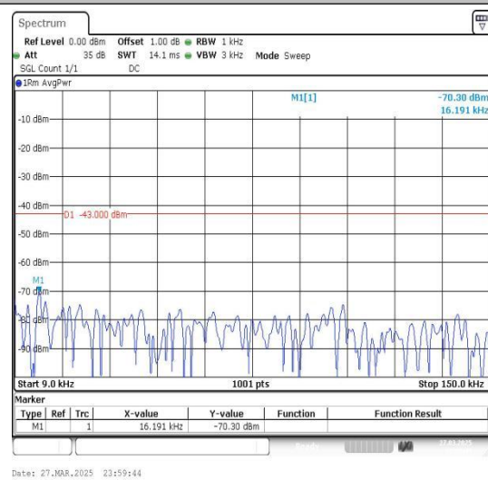
Band4_1.4MHz_QPSK_20393_1RB#0_0.009~0.15_0.009~0.15
