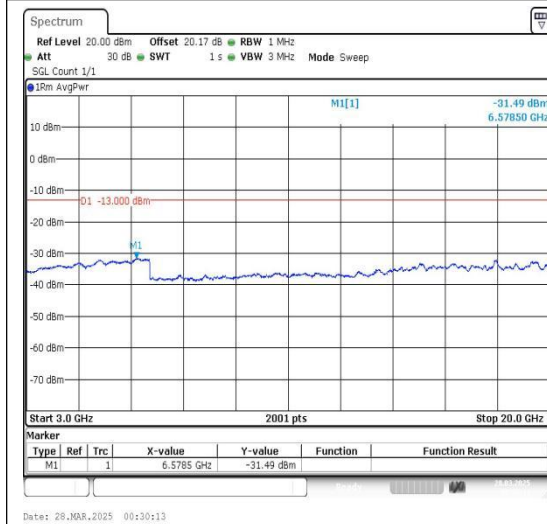
Band4_3MHz_QPSK_20385_1RB#0_3000~2000 0_3000~20000
