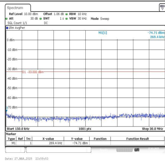
Band4_1.4MHz_QPSK_20393_1RB#0_0.15~30_0.15~30
