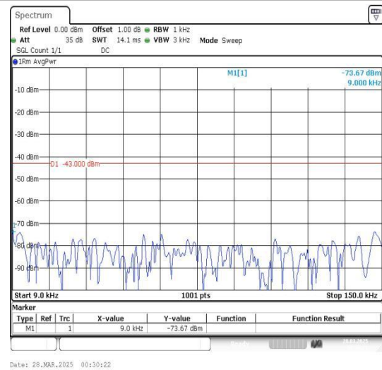
Band4_3MHz_16QAM_20385_1RB#0_0.009~0.15 _0.009~0.15
