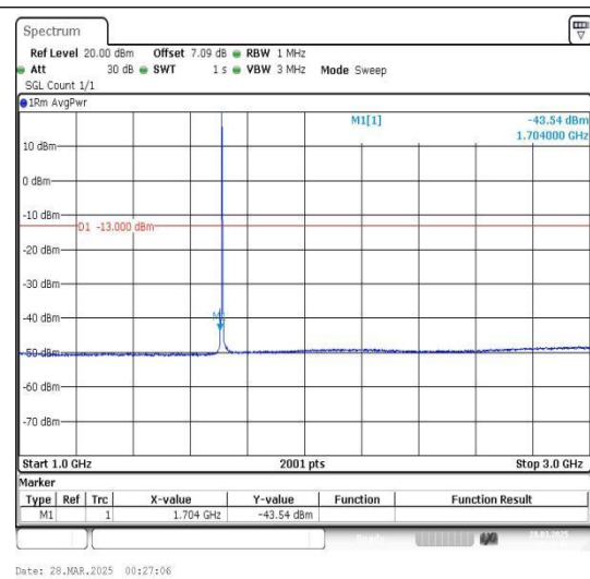
Band4_3MHz_QPSK_19965_1RB#0_1000~3000 1000~3000
