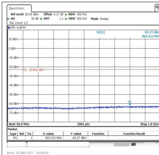
Band4_3MHz_QPSK_19965_1RB#0_30~1000_3 0~1000
