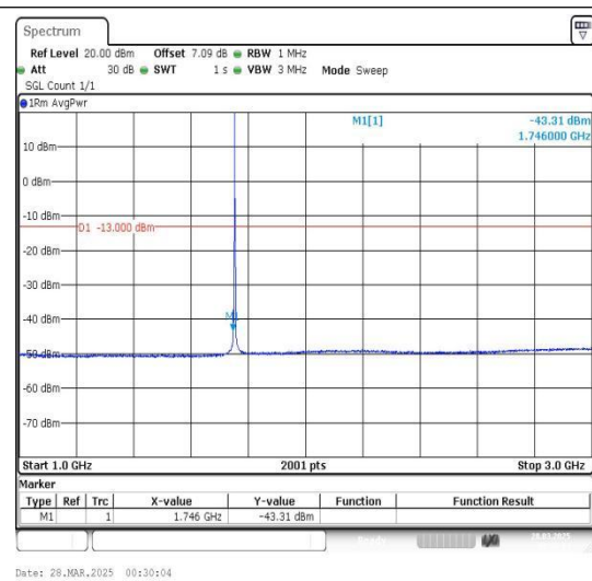
Band4_3MHz_QPSK_20385_1RB#0_1000~3000_1000~3000
