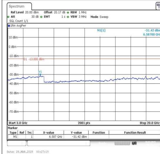
Band4_3MHz_QPSK_19965_1RB#0_3000~2000 0_3000~20000
