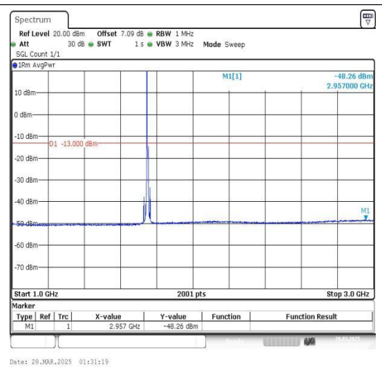
Band4_10MHz_QPSK_20350_1RB#0_1000~3000_1000~3000
