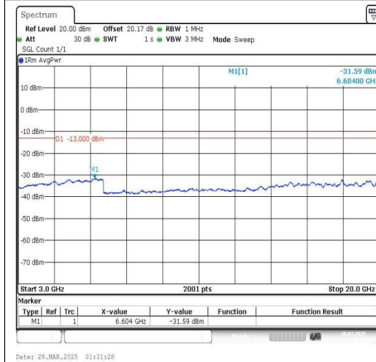
Band4_10MHz_QPSK_20350_1RB#0_3000~20000_3000~20000
