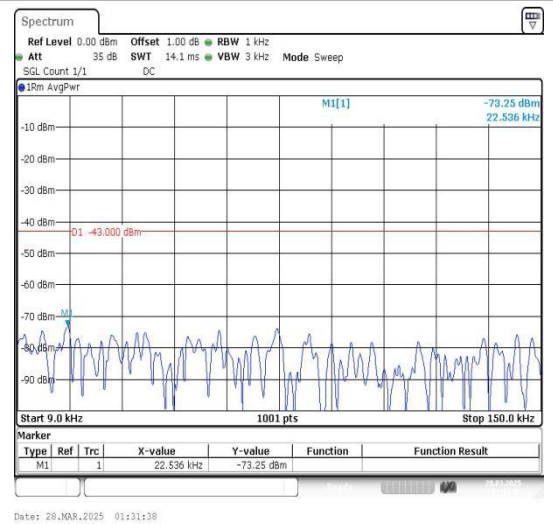
Band4_10MHz_16QAM_20350_1RB#0_0.009~0.15_0.009~0.15
