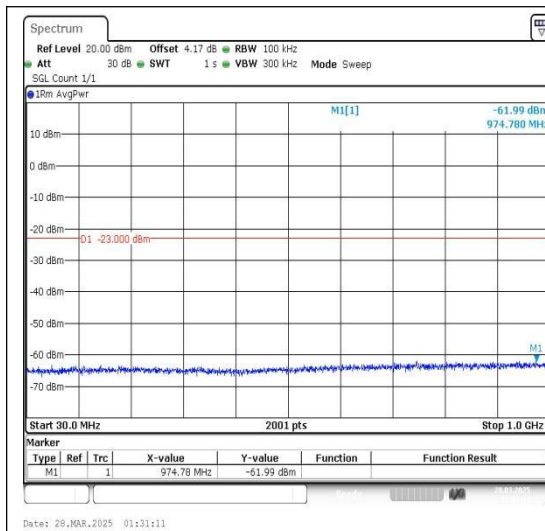
Band4_10MHz_QPSK_20350_1RB#0_30~1000_30~1000
