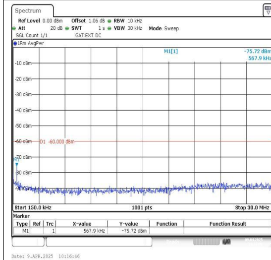
Band40_10MHz_QPSK_38750_1RB#0_0.15~3
