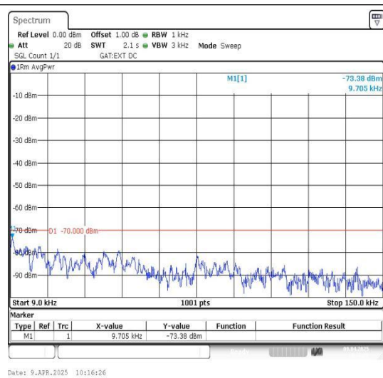
Band40_10MHz_16QAM_38750_1RB#0_0.009~0.15
