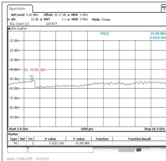
Band40_10MHz_QPSK_38750_1RB#0_3000~26500
