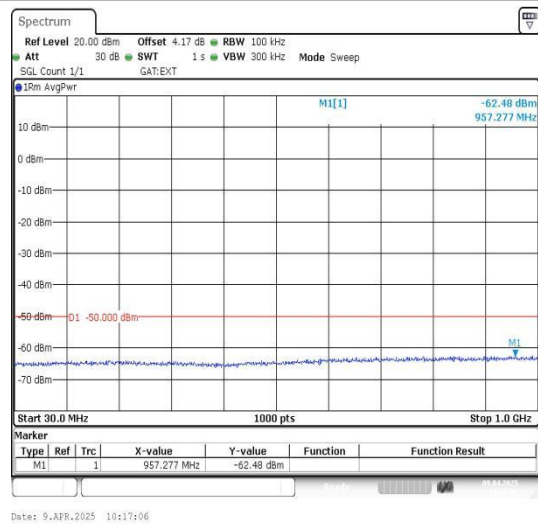
Band40_10MHz_16QAM_38750_1RB#0_30~1000
