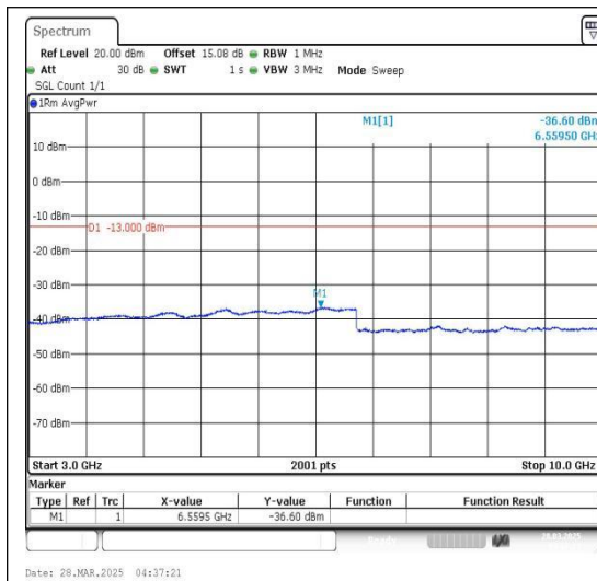
Band5_10MHz_QPSK_20525_1RB#0_3000~10000_3000~10000
