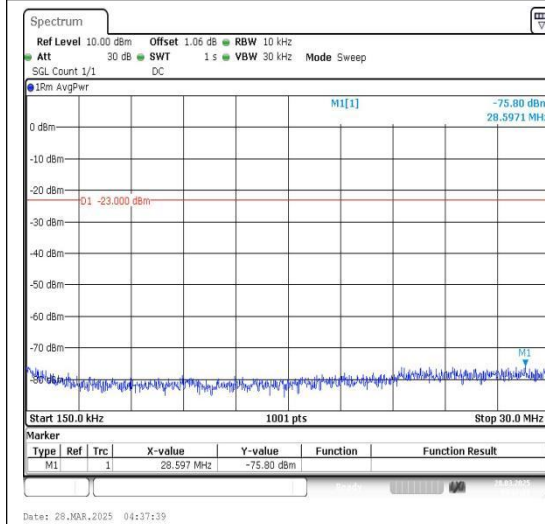
Band5_10MHz_16QAM_20525_1RB#0_0.15~30_0.15~30
