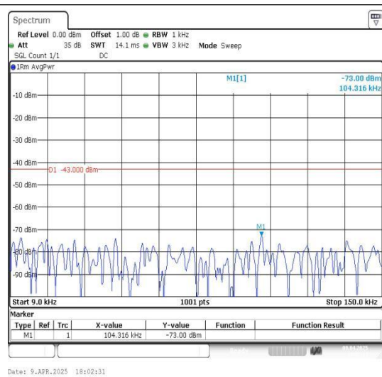
Band66_15MHz_16QAM_132322_1RB#0_0.009~0.15_0.009~0.15
