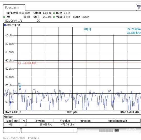
Band66_5MHz_16QAM_131997_1RB#0_0.009~0.15_0.009~0.15
