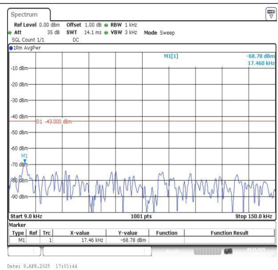
Band66_5MHz_16QAM_132322_1RB#0_0.009~0.15_0.009~0.15
