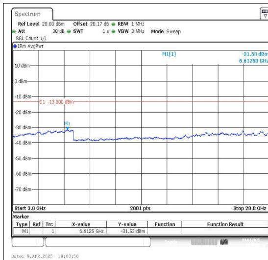
Band66_15MHz_QPSK_132047_1RB#0_3000~20000
