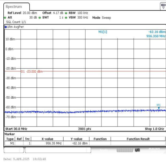
Band66_15MHz_16QAM_132322_1RB#0_30~100_30~1000
