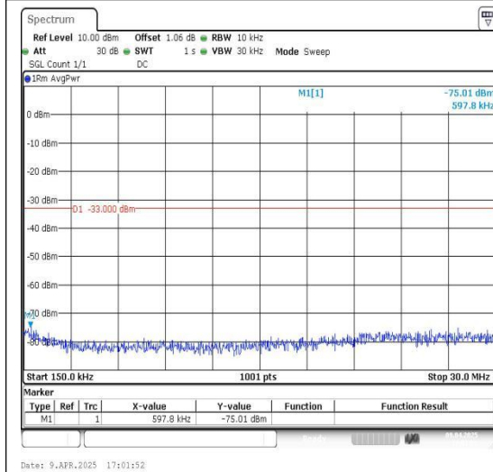
Band66_5MHz_16QAM_132322_1RB#0_0.15~30_0.15~30
