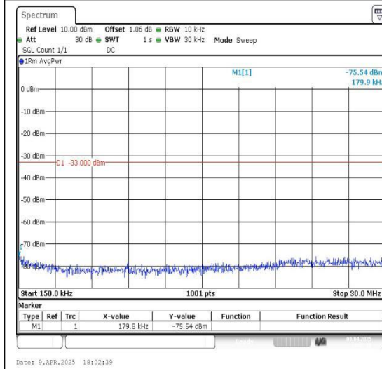
Band66_15MHz_QPSK_132322_1RB#0_0.15~30_0.15~30
