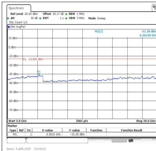
Band66_15MHz_QPSK_132322_1RB#0_3000~20000_3000~20000
