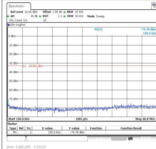
Band66_10MHz_16QAM_132022_1RB#0_0.15~30_0.15~30
