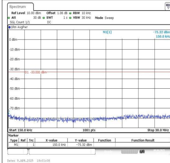
Band66_15MHz_QPSK_132047_1RB#0_0.15~30
