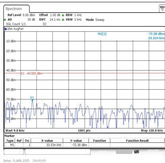
Band66_15MHz_16QAM_132047_1RB#0_0.009~0.15
