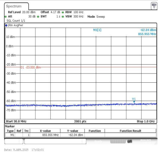
Band66_5MHz_16QAM_132322_1RB#0_30~1000_30~1000
