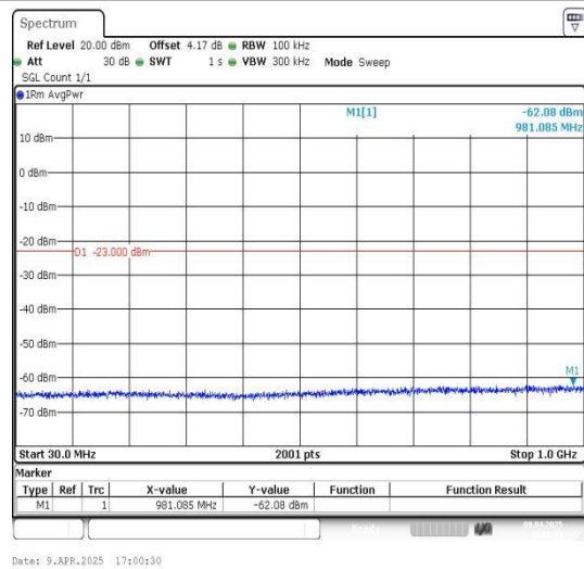
Band66_5MHz_16QAM_131997_1RB#0_30~1000_30~1000
