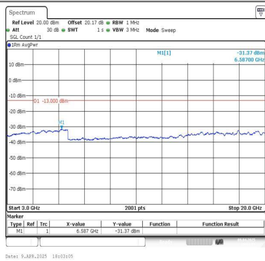
Band66_15MHz_16QAM_132322_1RB#0_30~100_30~1000
