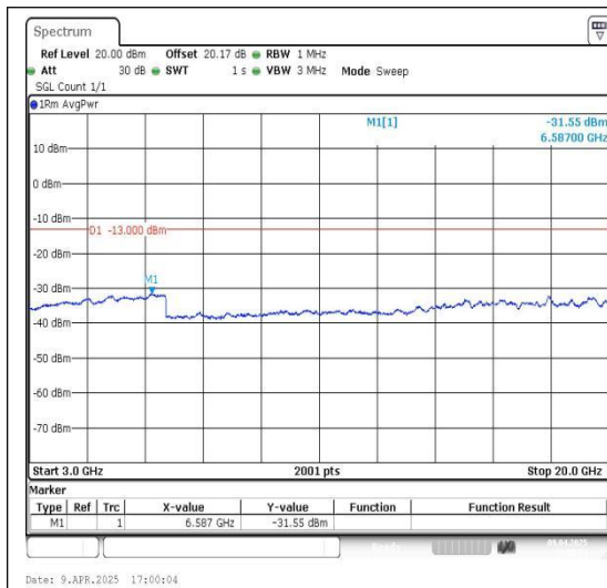
Band66_5MHz_QPSK_131997_1RB#0_3000~20000
