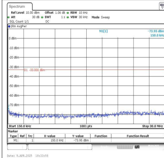
Band66_20MHz_QPSK_132322_1RB#0_0.15~30_0.15~30
