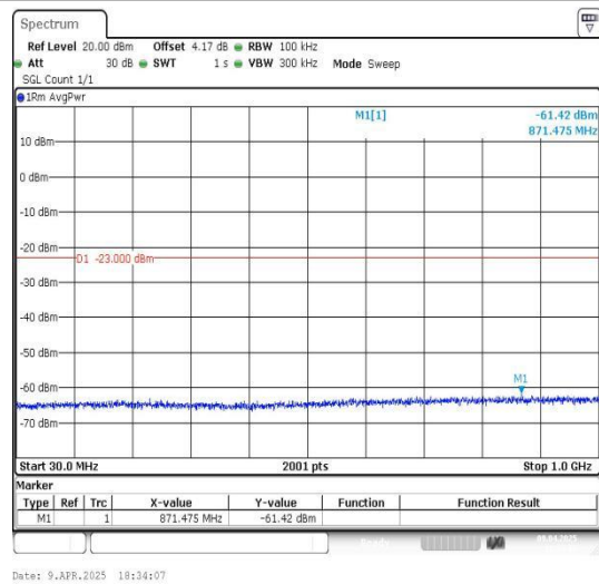
Band66_20MHz_16QAM_132322_1RB#0_30~100_30~1000
