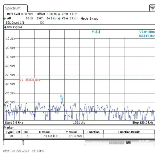
Band7_10MHz_16QAM_21400_1RB#0_0.009~0.1 5_0.009~0.15
