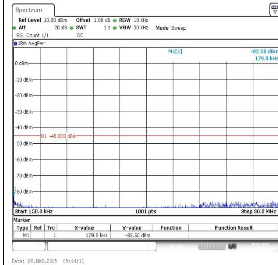
Band7_10MHz_16QAM_21400_1RB#0_0.15~30 _0.15~30
