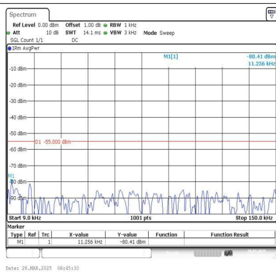
Band7_20MHz_16QAM_20850_1RB#0_0.009~0.15_5_0.009~0.15
