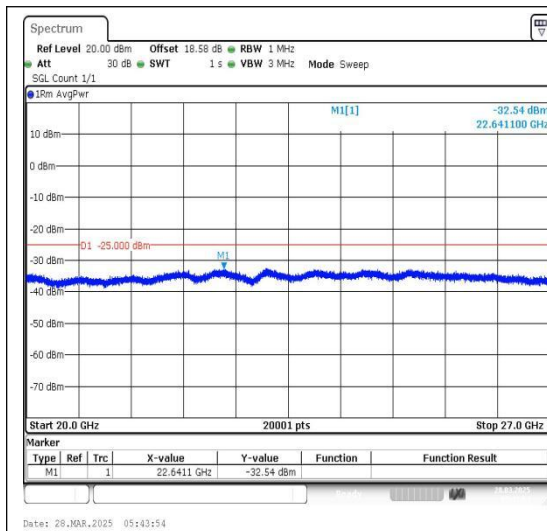
Band7_10MHz_QPSK_21400_1RB#0_20000~27000
