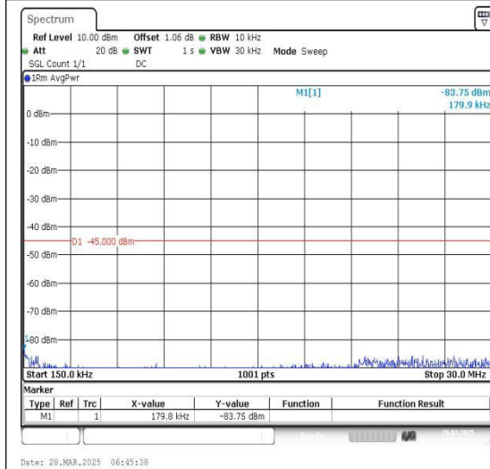
Band7_20MHz_16QAM_20850_1RB#0_0.15~30_0.15~30
