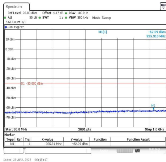
Band7_20MHz_16QAM_20850_1RB#0_30~1000_30~1000
