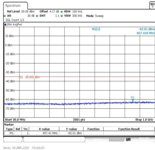
Band7_10MHz_16QAM_21400_1RB#0_30~1000 30~1000
