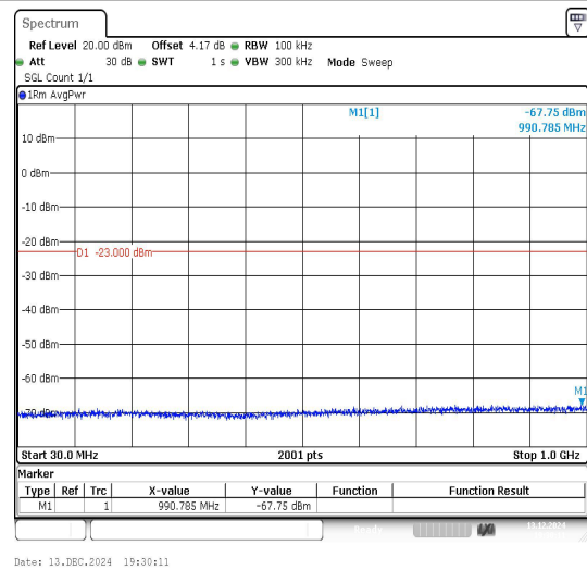
Band2_10MHz_16QAM_18650_1RB#0_30~1000_30~1000
