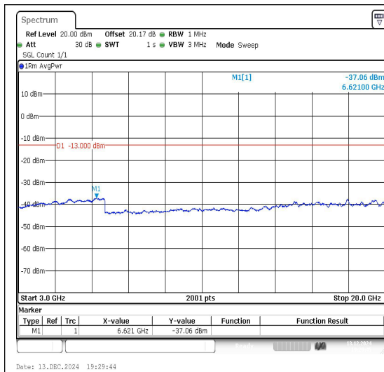
Band2_10MHz_QPSK_18650_1RB#0_3000~20000_3000~20000
