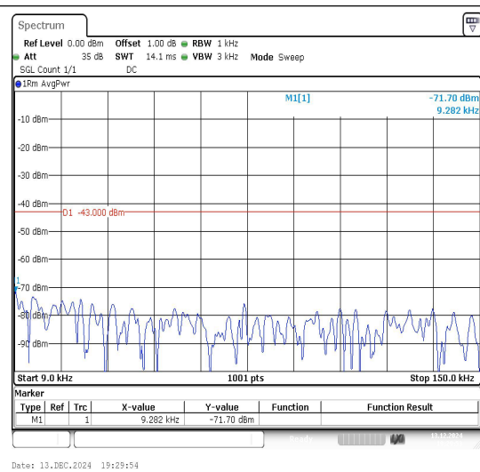
Band2_10MHz_16QAM_18650_1RB#0_0.009~0.15_0.009~0.15
