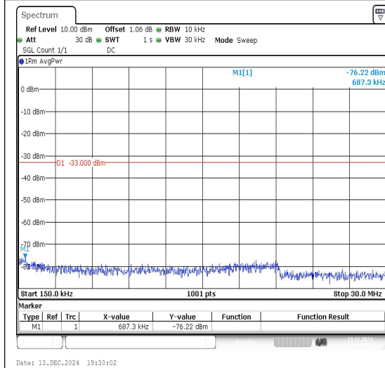
Band2_10MHz_16QAM_18650_1RB#0_0.15~30_0.15~30
