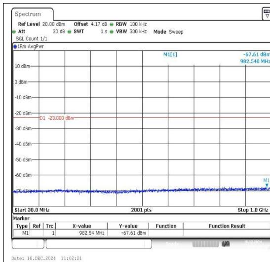
Band66_1.4MHz_QPSK_132322_1RB#0_30~100 0_30~1000
