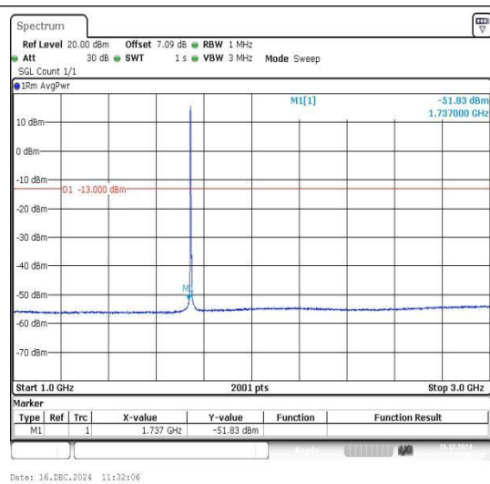
Band66_3MHz_QPSK_132322_1RB#0_1000~3000_0_1000~3000
