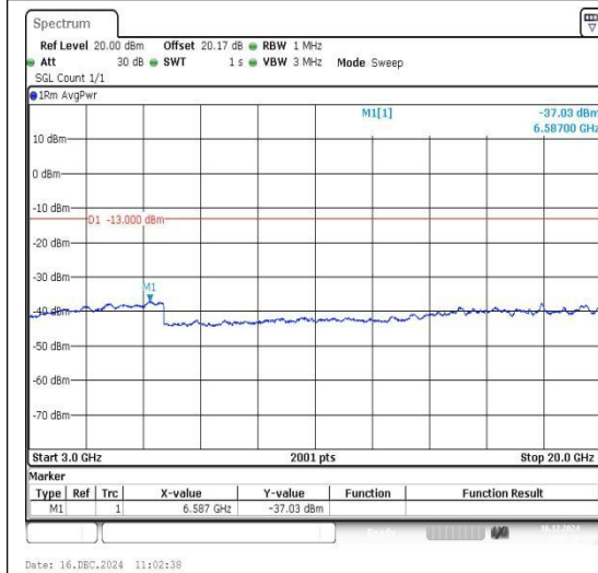
Band66_1.4MHz_QPSK_132322_1RB#0_3000~2 0000_3000~20000
