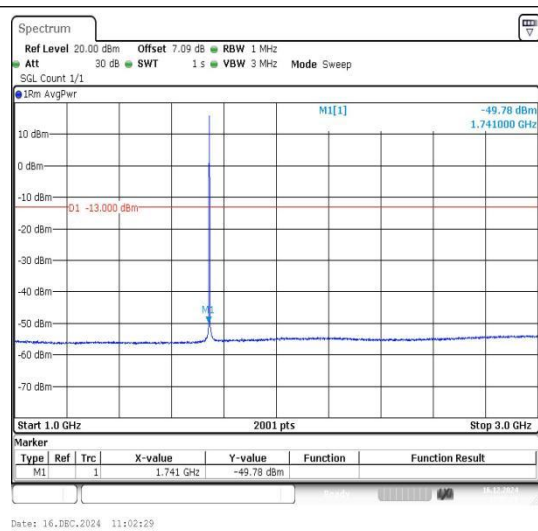
Band66_1.4MHz_QPSK_132322_1RB#0_1000~3 000_1000~3000
