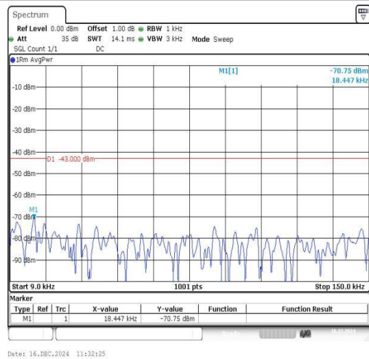
Band66_3MHz_16QAM_132322_1RB#0_0.009~0.15_15_0.009~0.15
