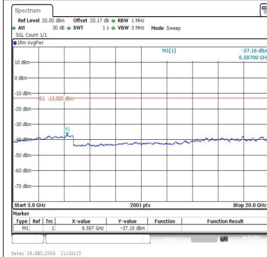
Band66_3MHz_QPSK_132322_1RB#0_3000~20000_000_3000~20000
