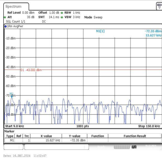
Band66_1.4MHz_16QAM_132322_1RB#0_0.009~ 0.15_0.009~0.15
