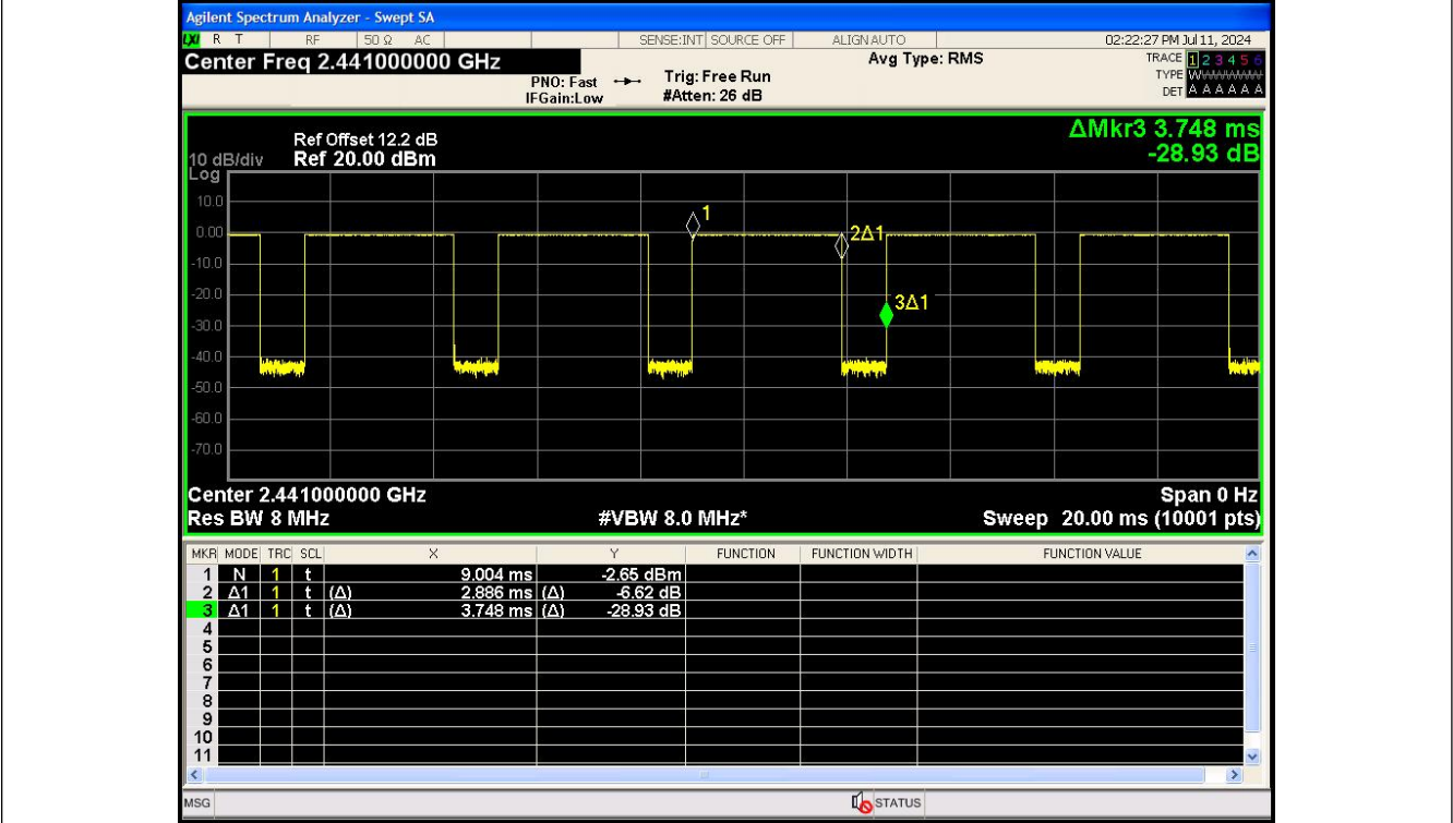
GFSK(DH5)_Channel 39
