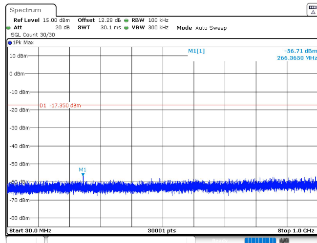
Thread_Ant1_2405_0~Reference
