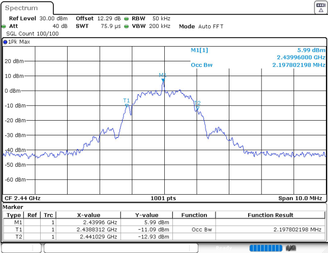
Thread_Ant1_2440
