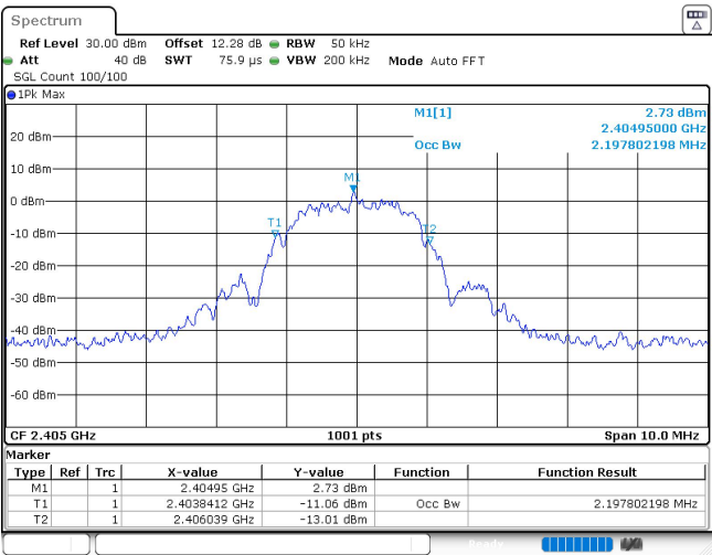
Thread_Ant1_2405
