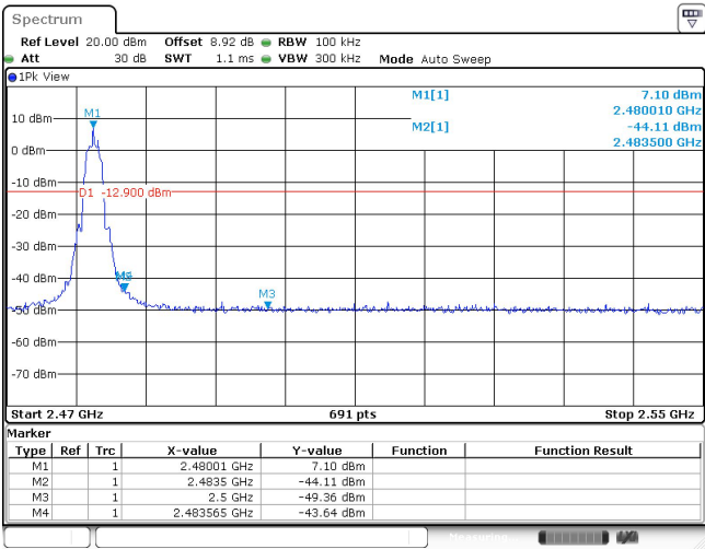
Thread_Ant1_High_2480
