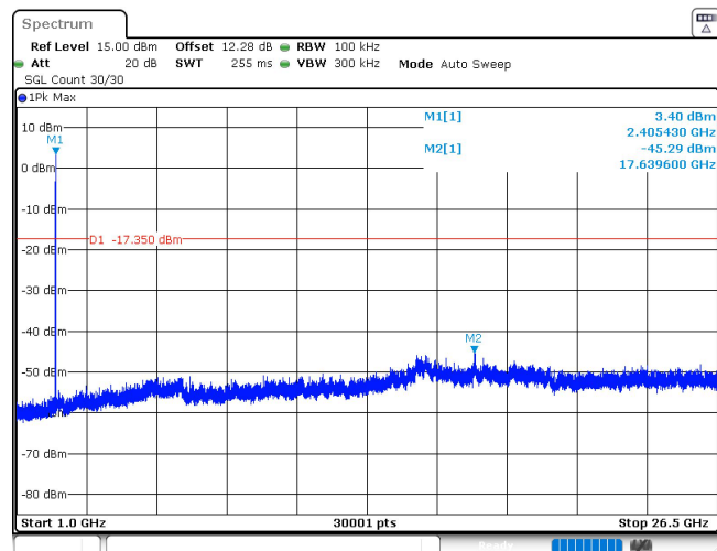
Thread_Ant1_2405_1000~26500
