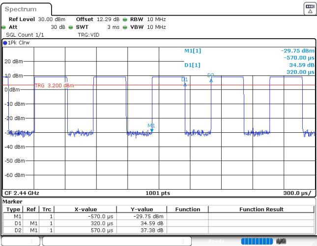
Thread_Ant1_2440
