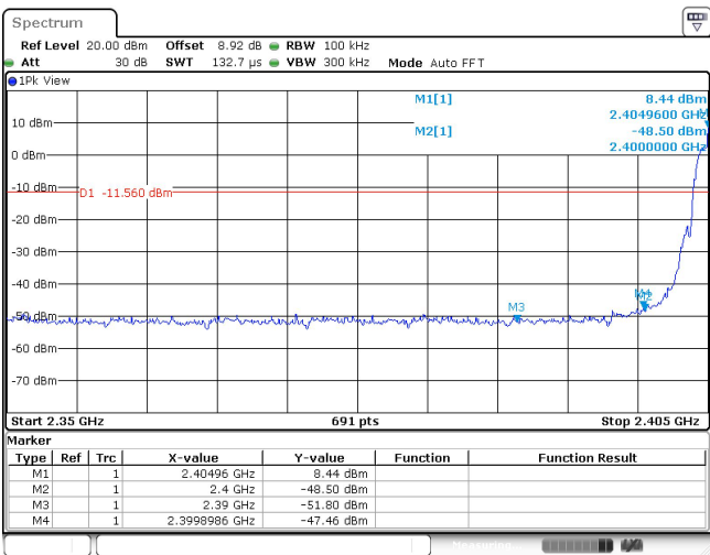
Thread_Ant1_Low_2405
